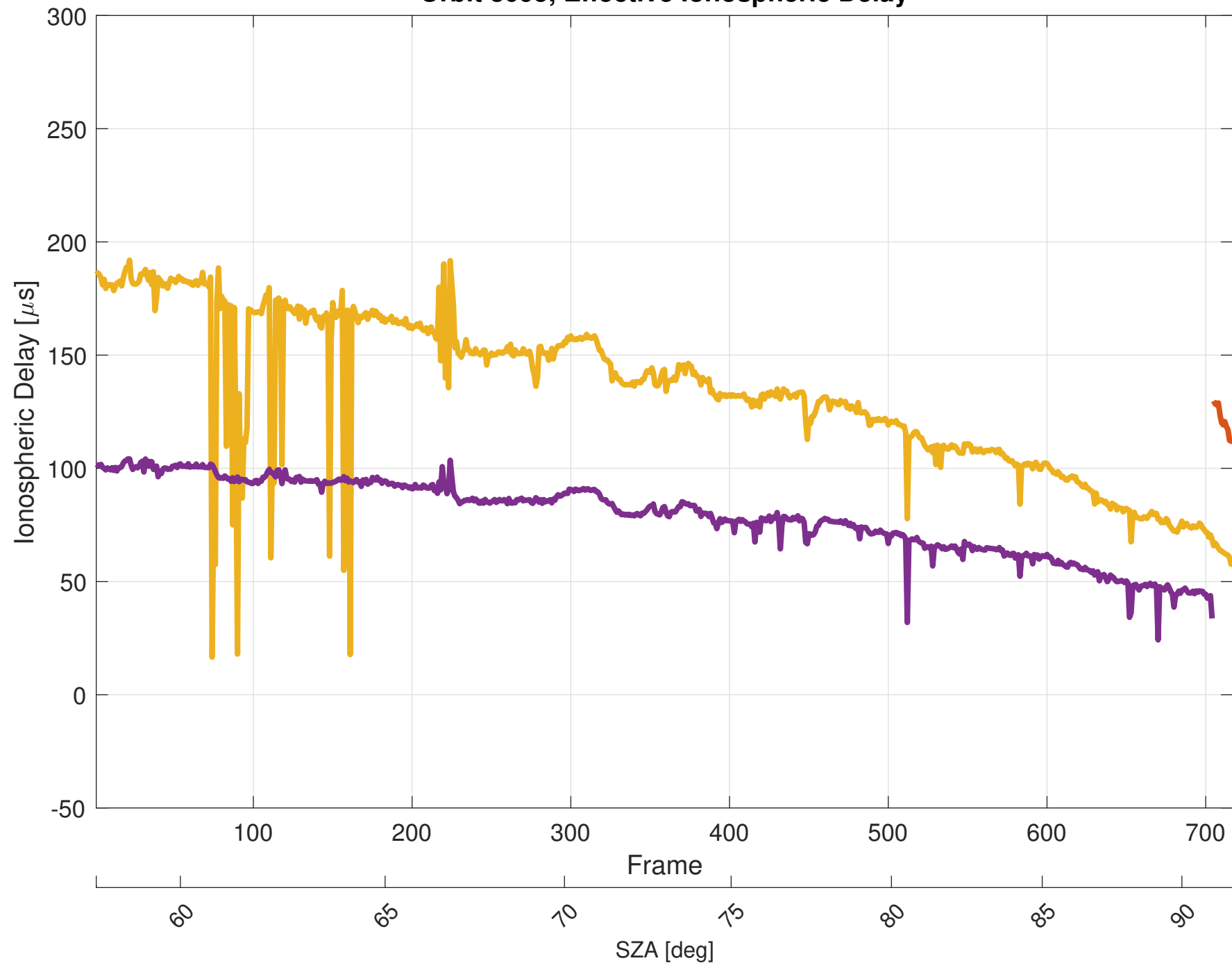
Orbit 3095, Effective Ionospheric Delay
