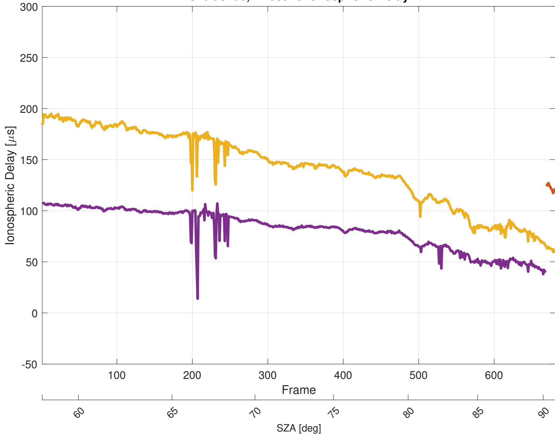
Orbit 3100, Effective Ionospheric Delay
