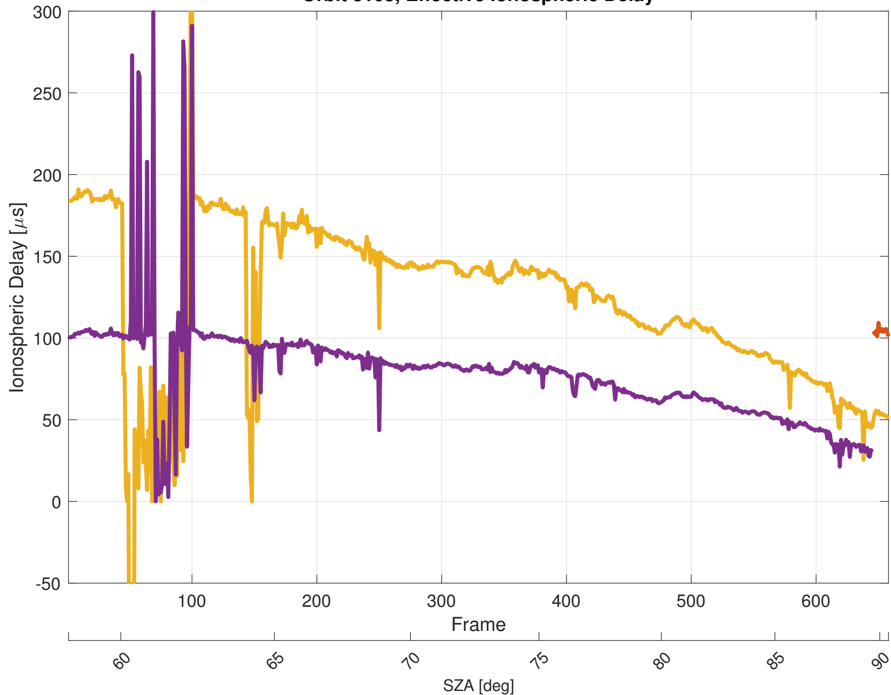
Orbit 3103, Effective Ionospheric Delay
