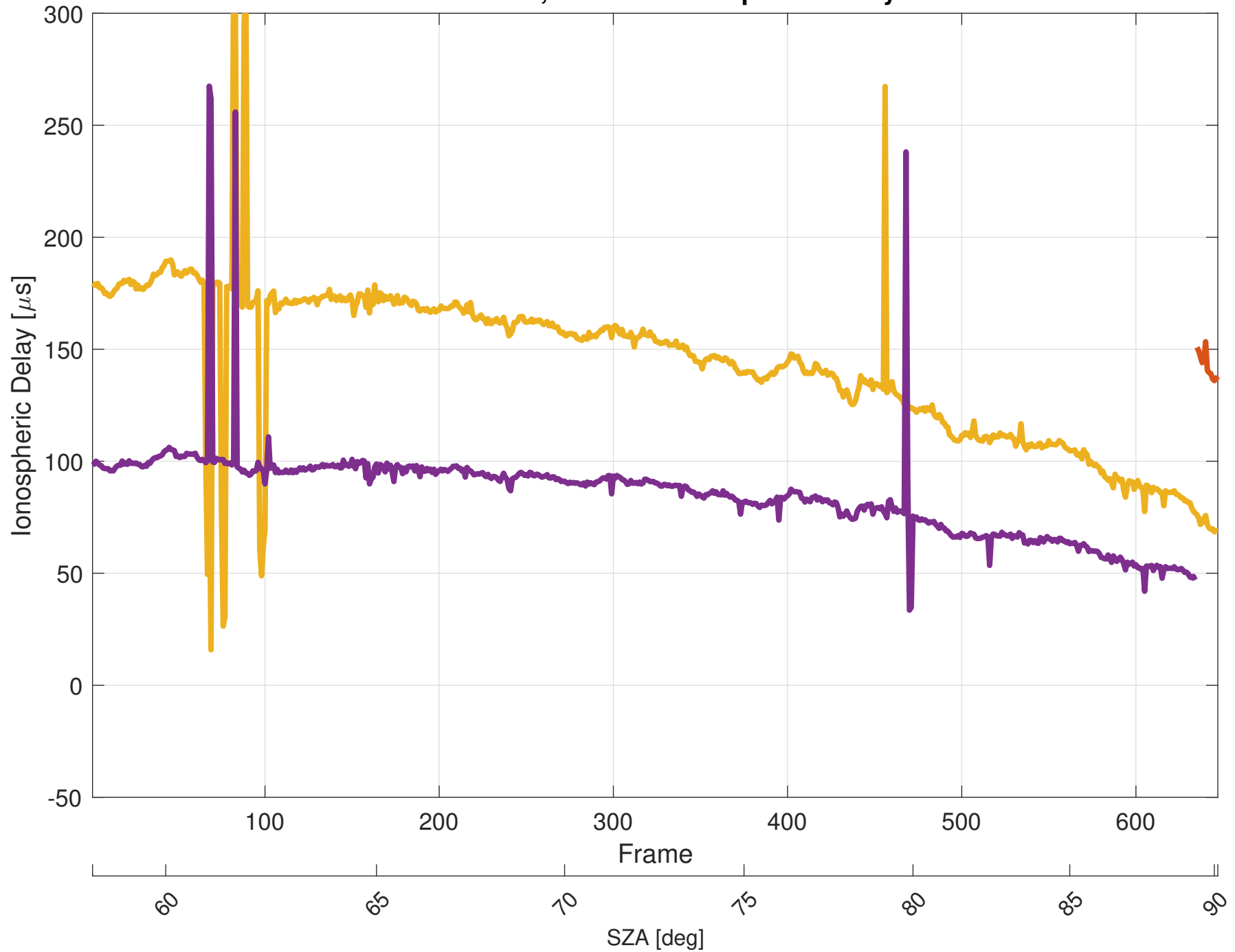
Orbit 3105, Effective Ionospheric Delay
