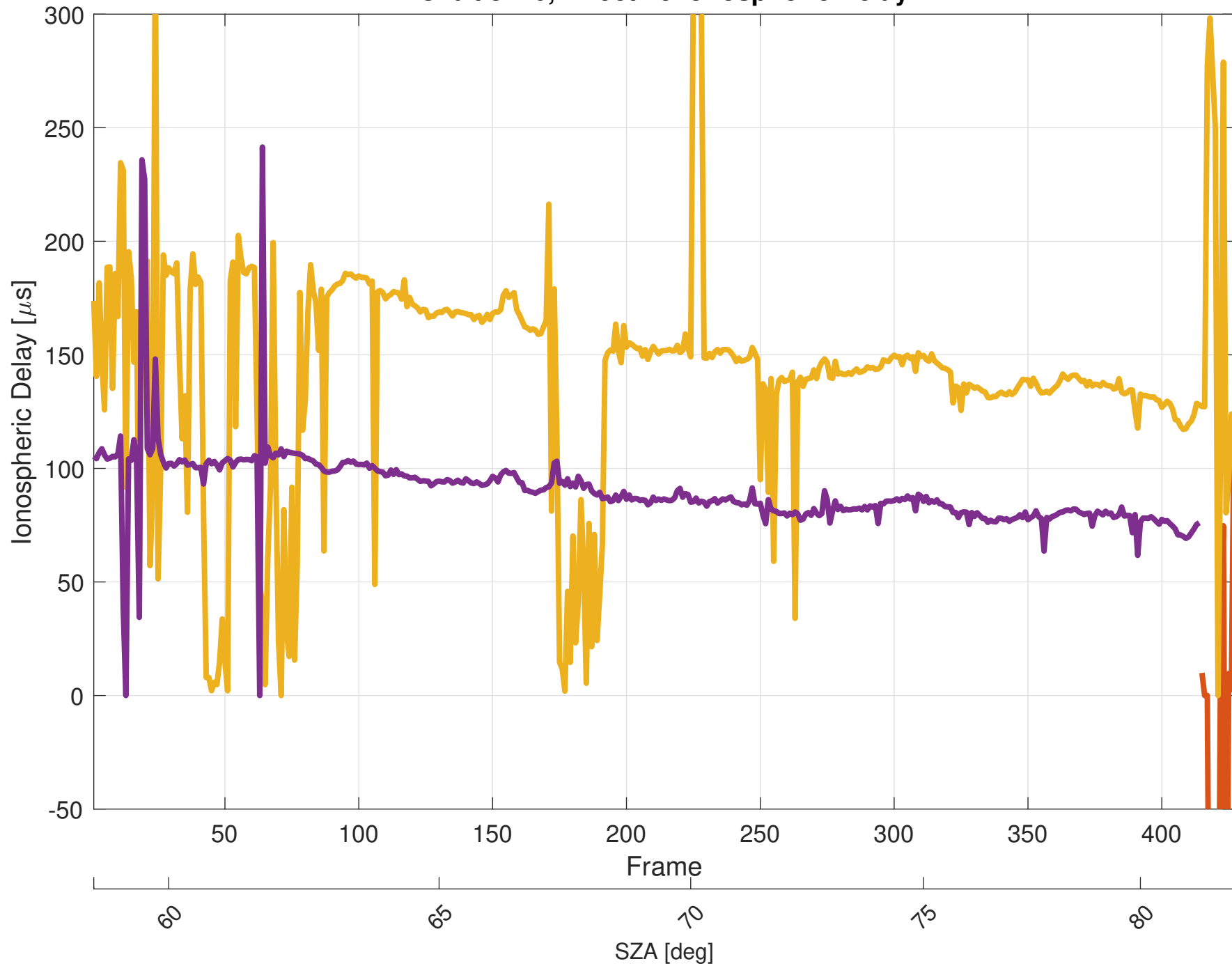
Orbit 3146, Effective Ionospheric Delay
