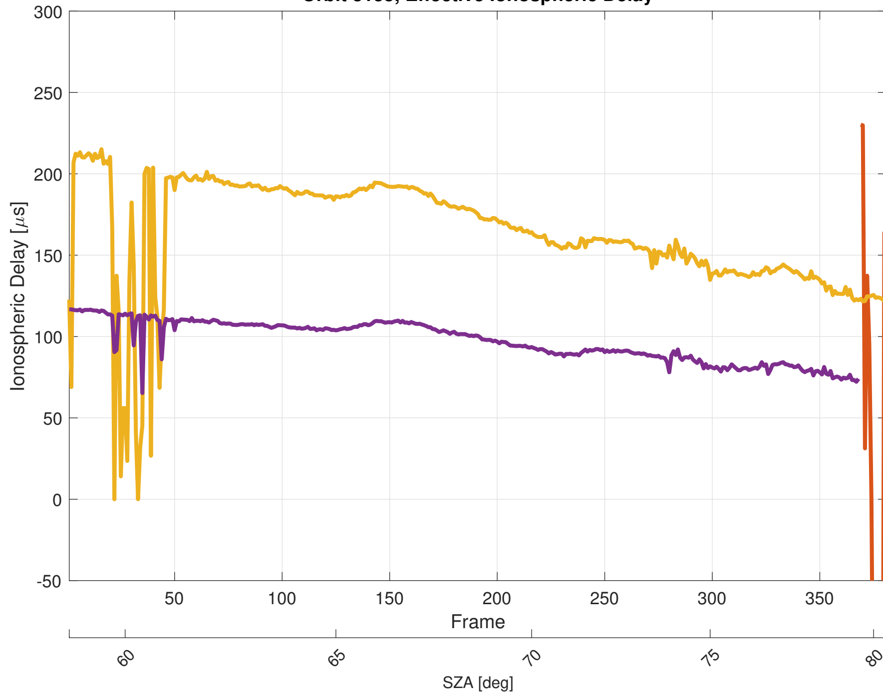
Orbit 3155, Effective Ionospheric Delay
