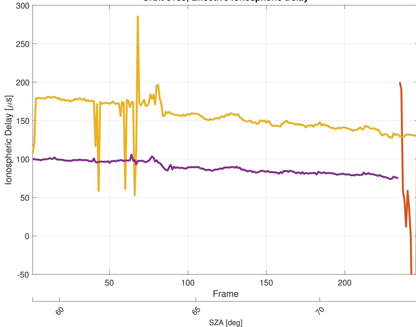
Orbit 3183, Effective Ionospheric Delay
