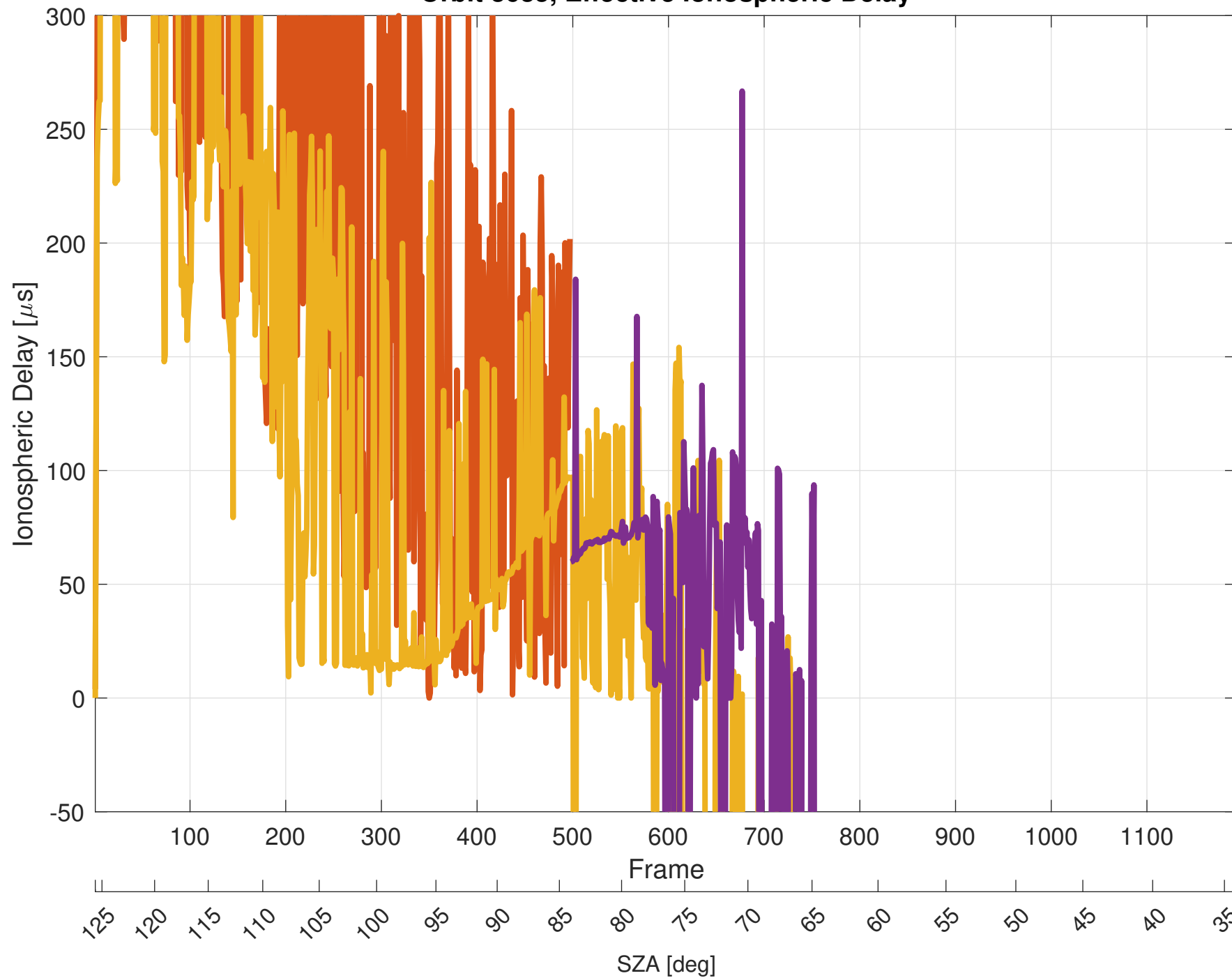
Orbit 3635, Effective Ionospheric Delay
