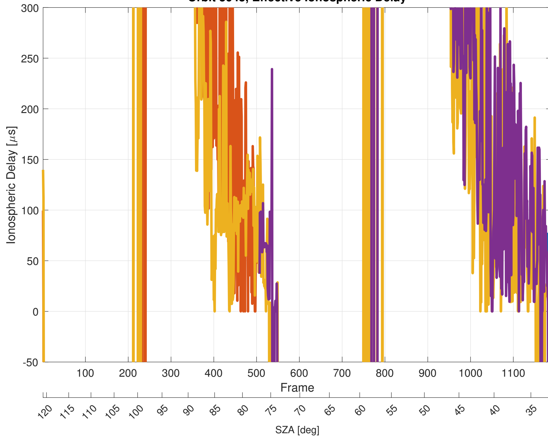
Orbit 3643, Effective Ionospheric Delay
