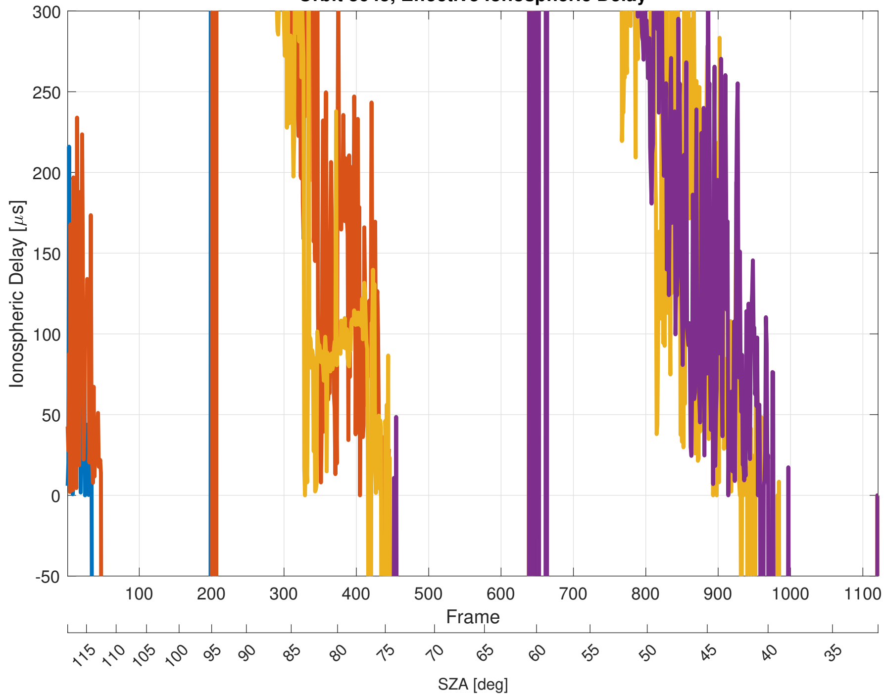
Orbit 3645, Effective Ionospheric Delay
