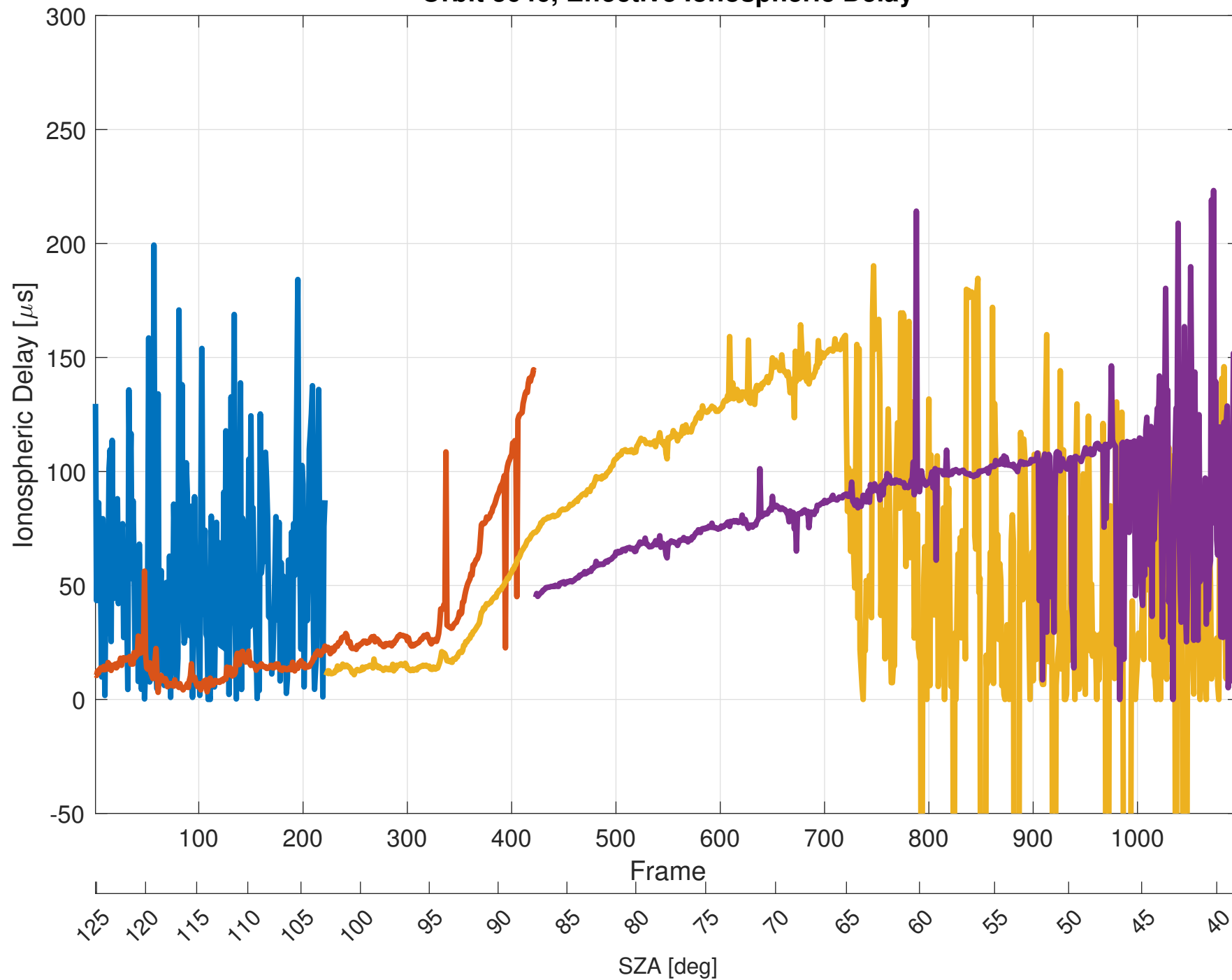
Orbit 3646, Effective Ionospheric Delay
