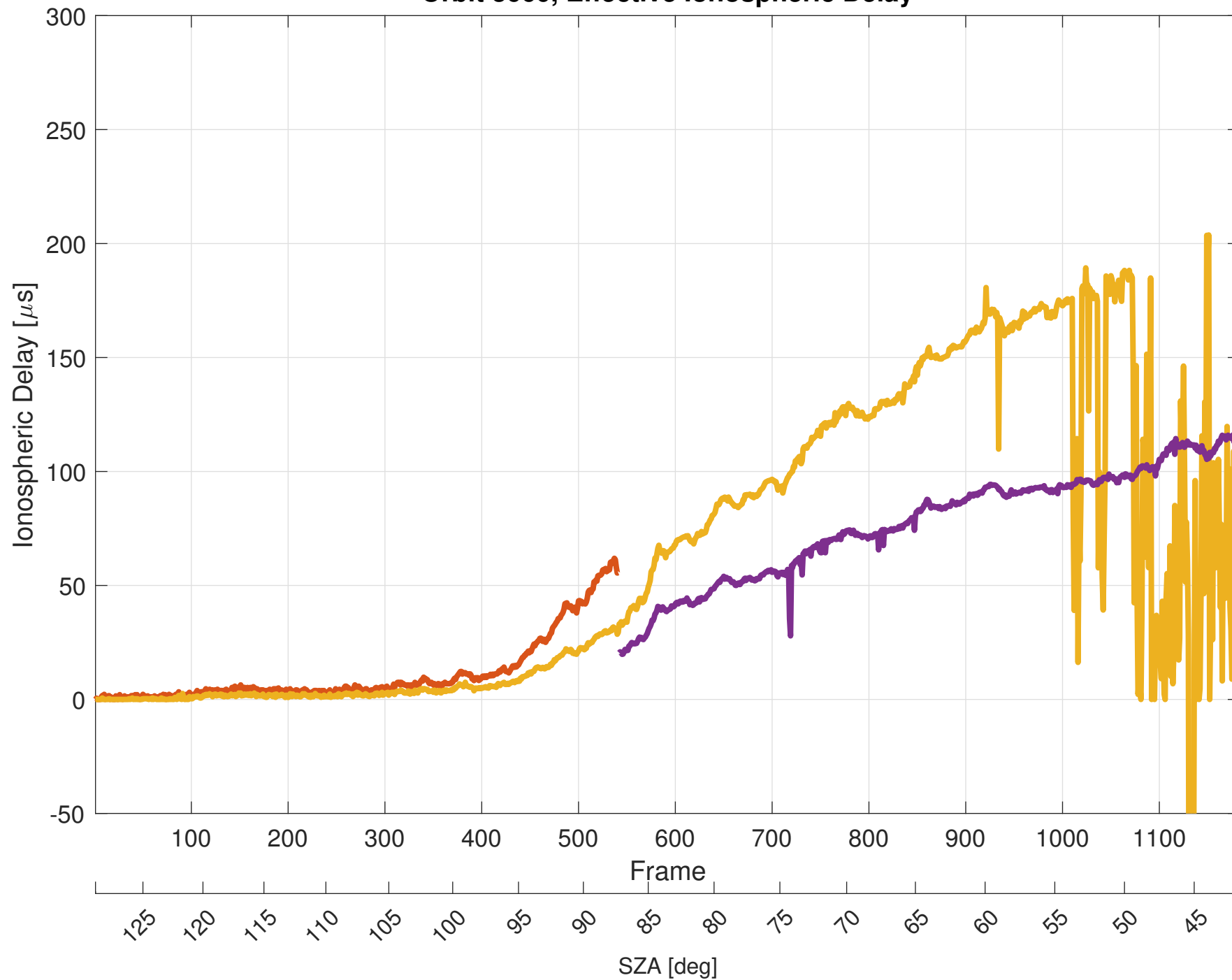
Orbit 3660, Effective Ionospheric Delay
