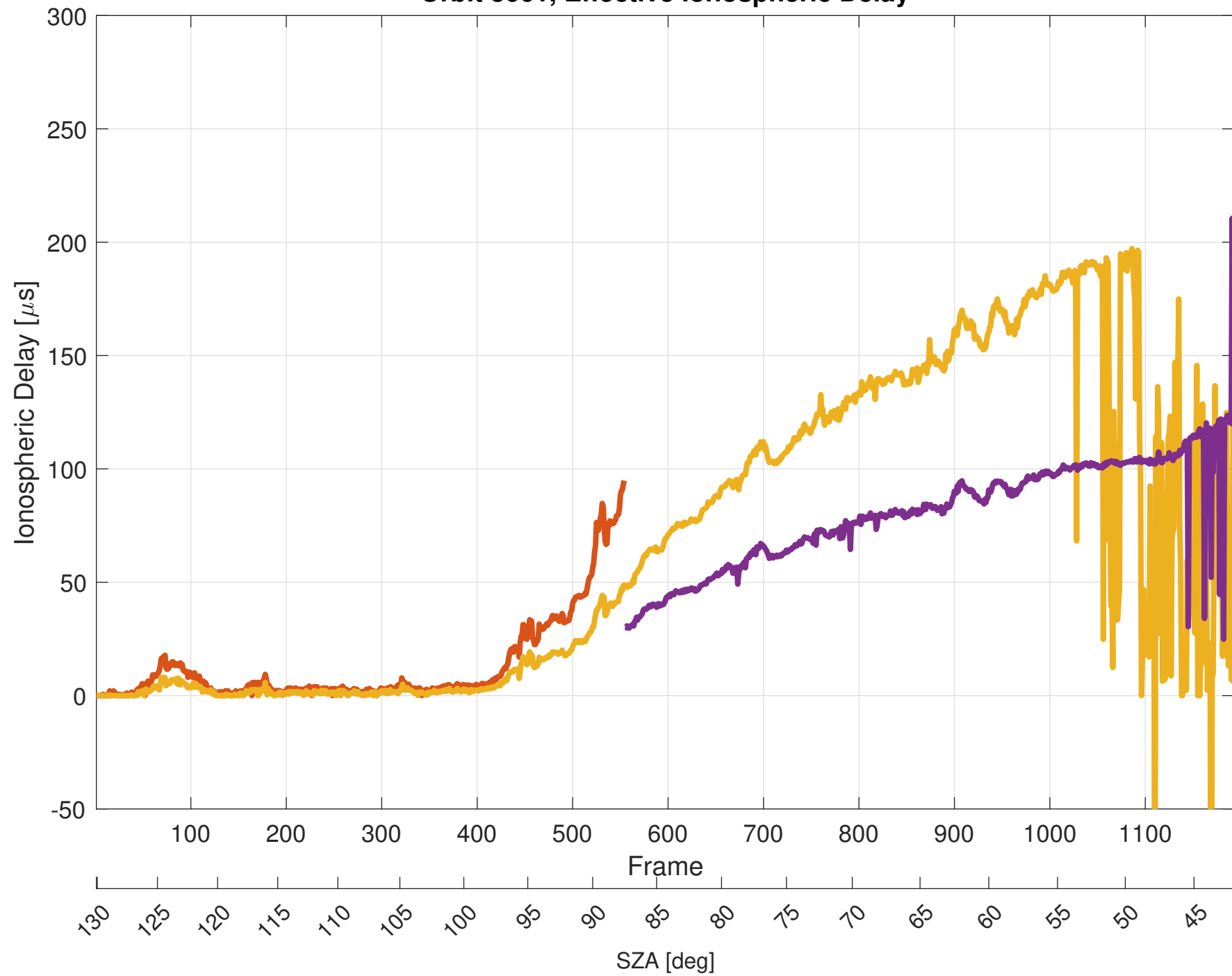
Orbit 3661, Effective Ionospheric Delay
