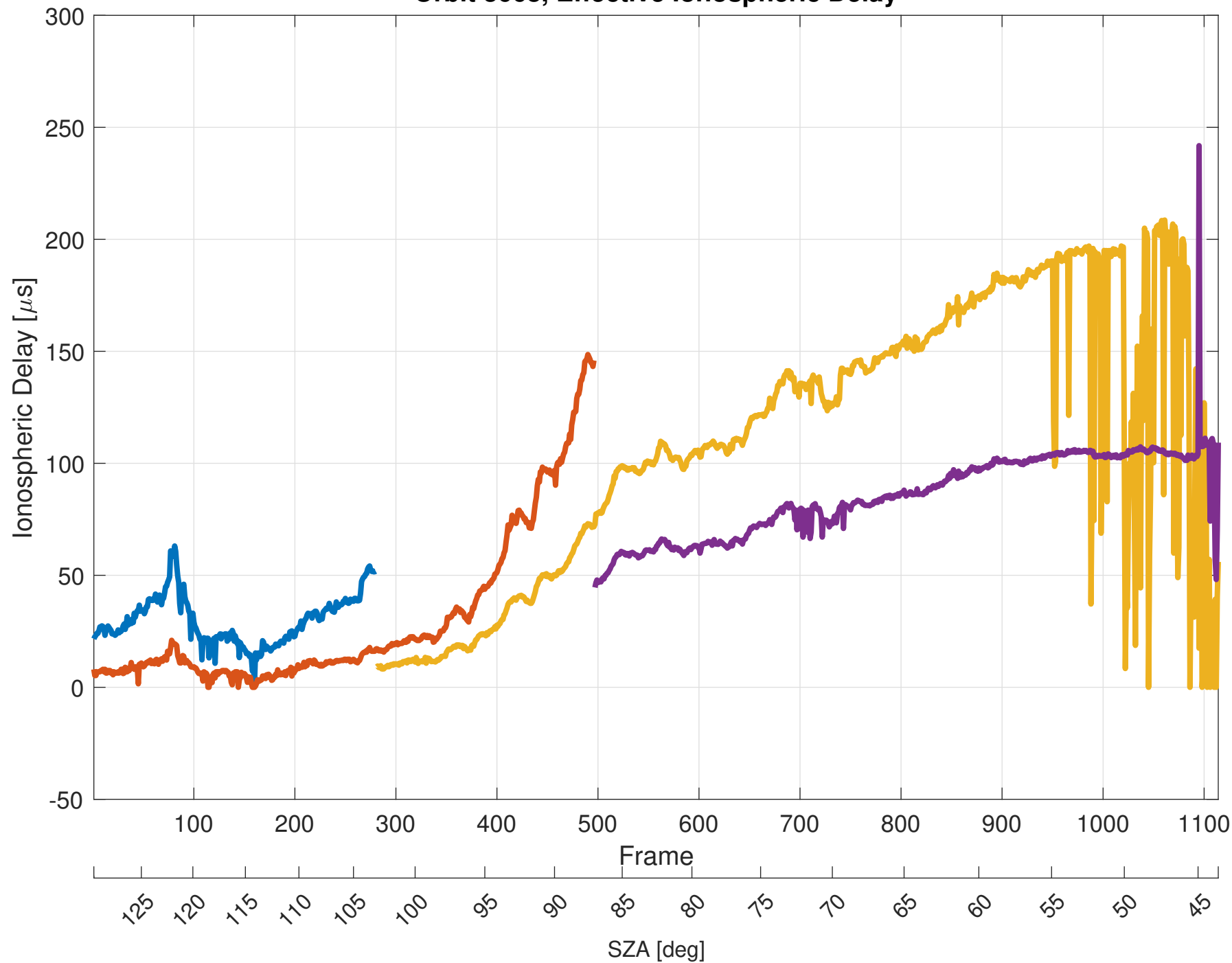
Orbit 3668, Effective Ionospheric Delay
