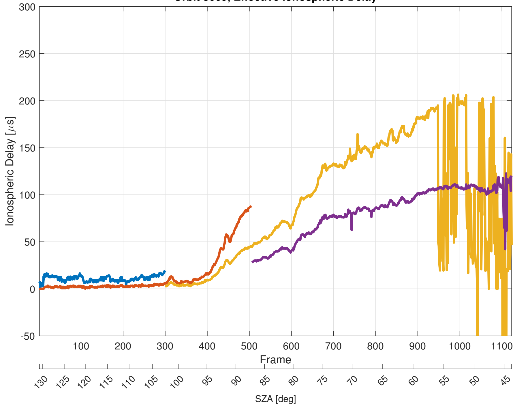
Orbit 3669, Effective Ionospheric Delay
