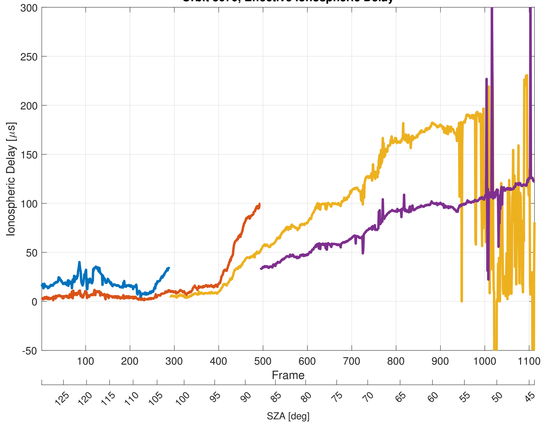
Orbit 3670, Effective Ionospheric Delay
