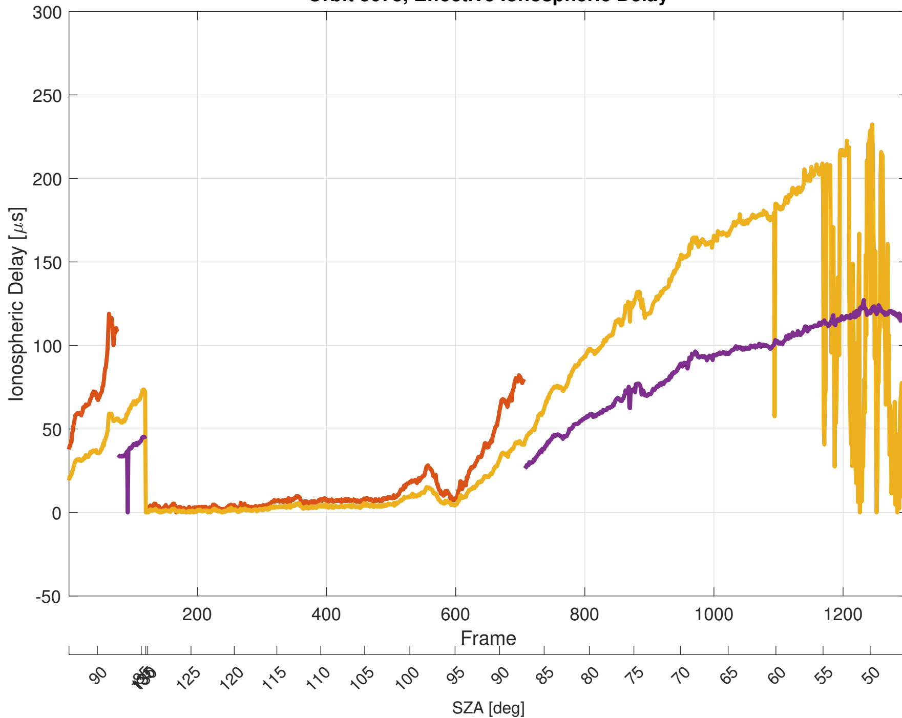
Orbit 3678, Effective Ionospheric Delay
