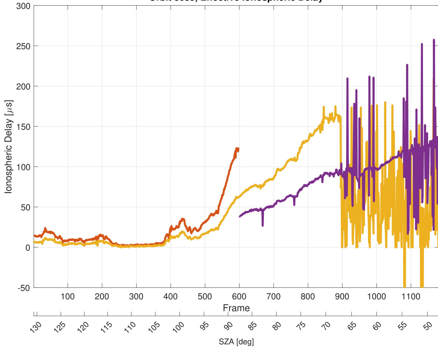
Orbit 3685, Effective Ionospheric Delay
