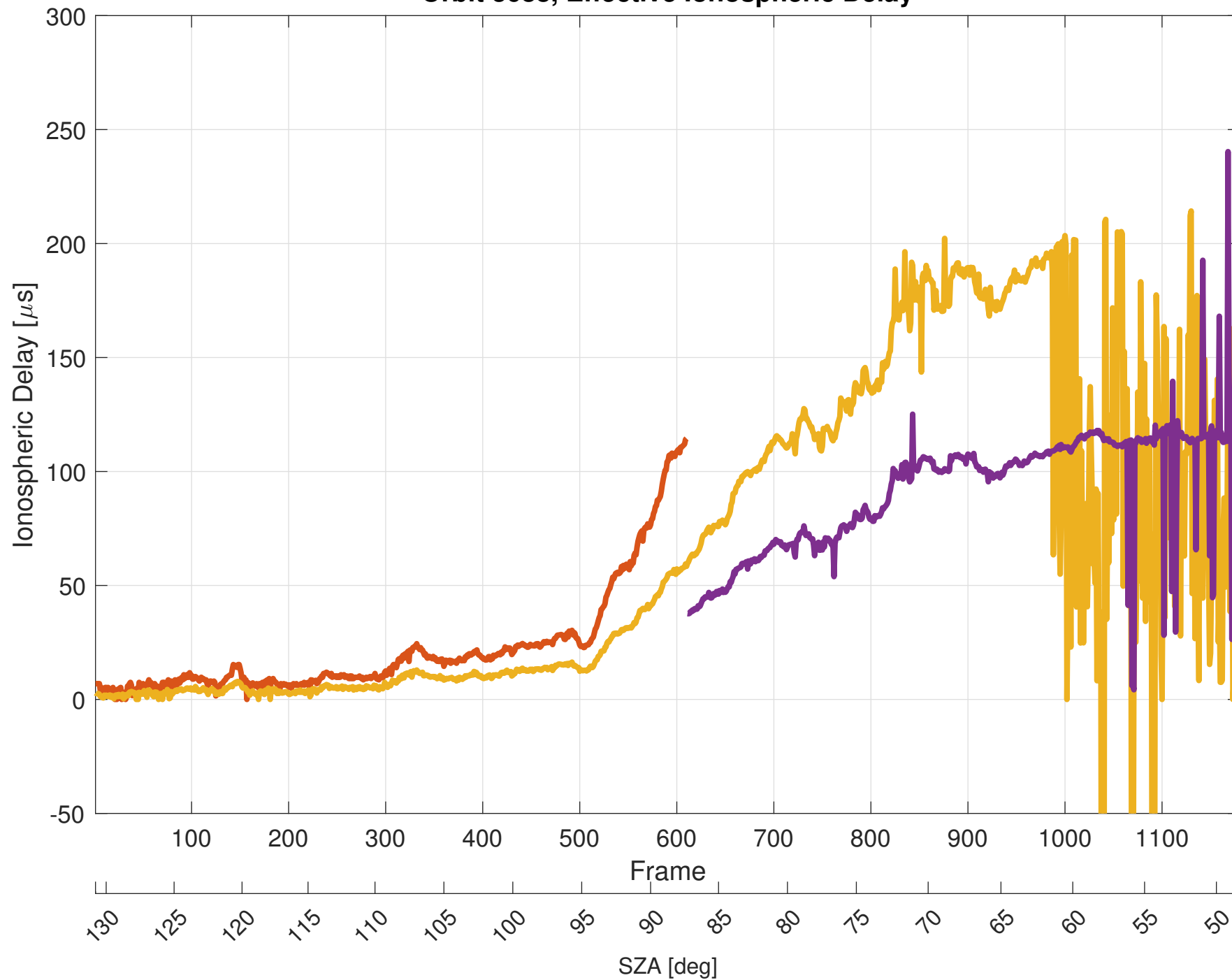
Orbit 3688, Effective Ionospheric Delay
