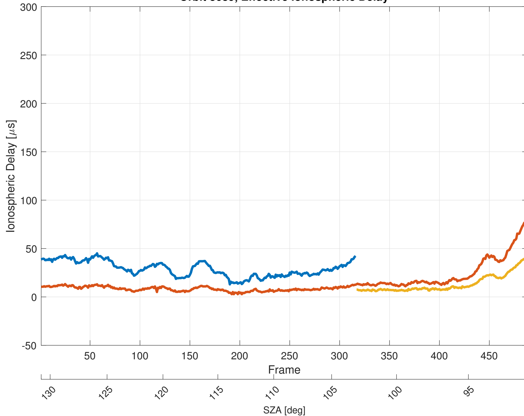
Orbit 3689, Effective Ionospheric Delay
