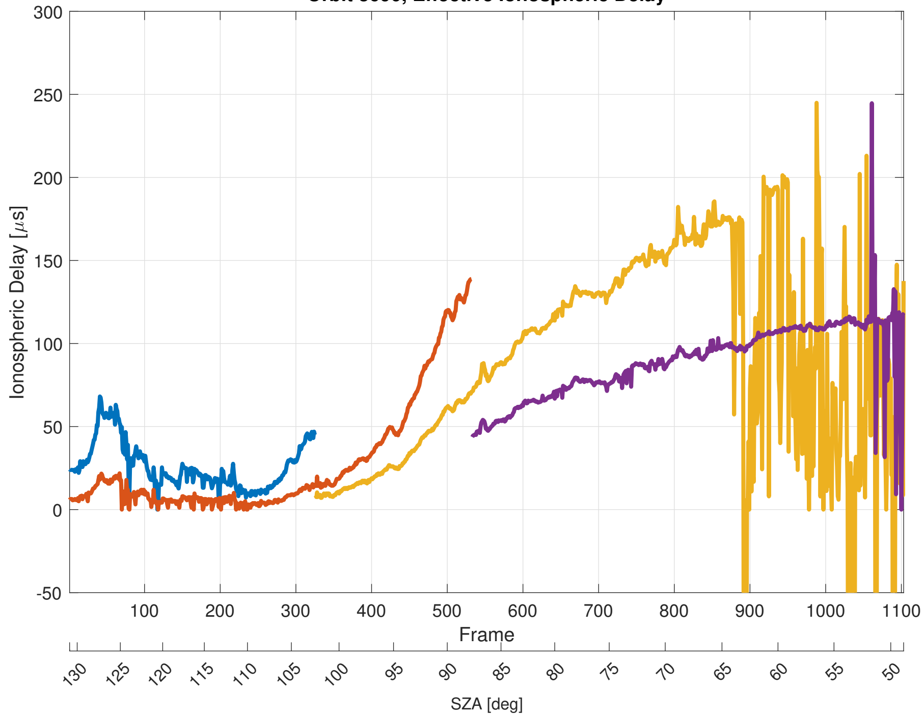
Orbit 3690, Effective Ionospheric Delay
