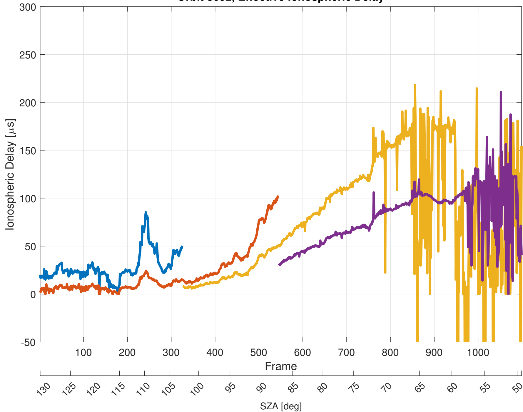
Orbit 3692, Effective Ionospheric Delay
