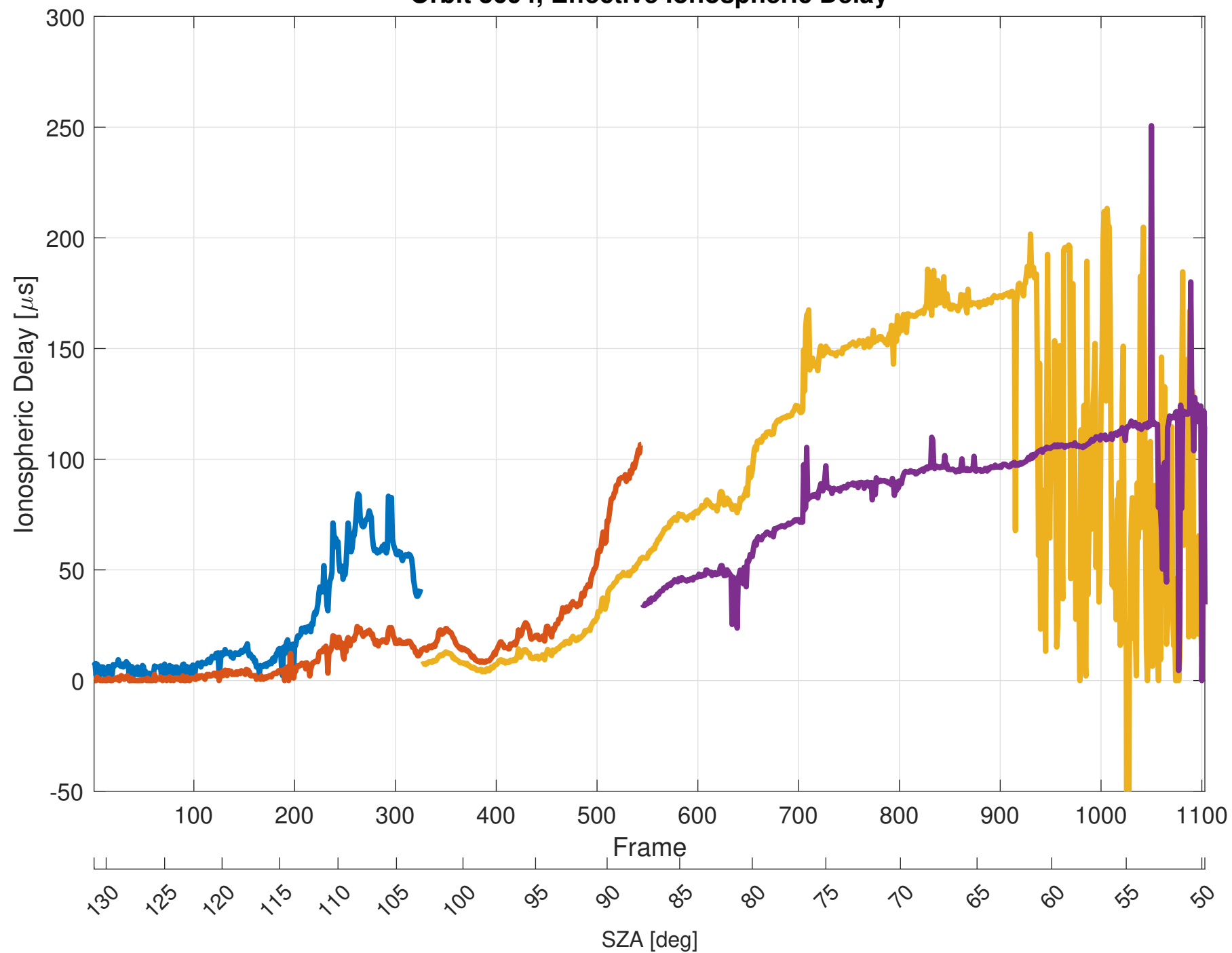
Orbit 3694, Effective Ionospheric Delay
