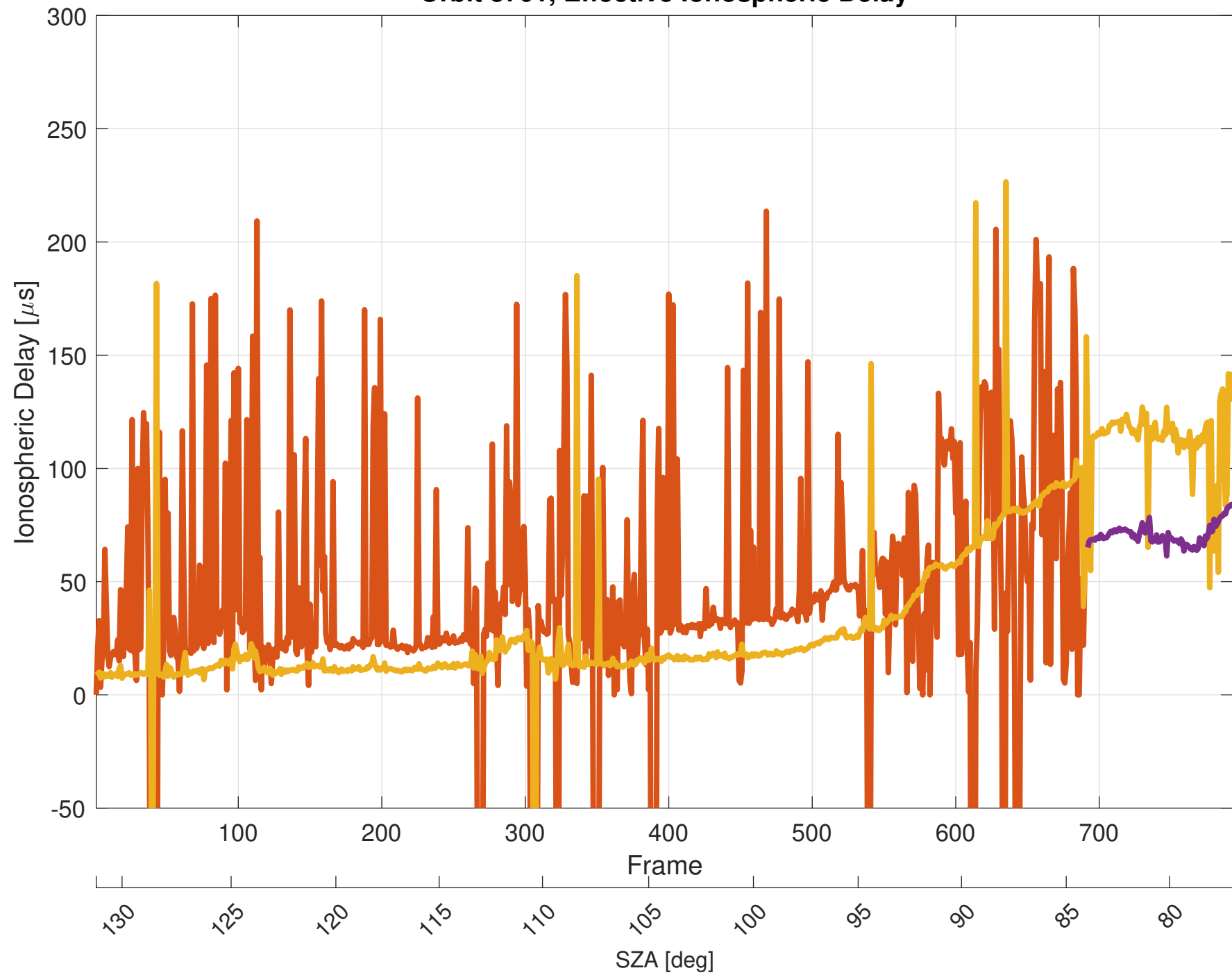
Orbit 3701, Effective Ionospheric Delay
