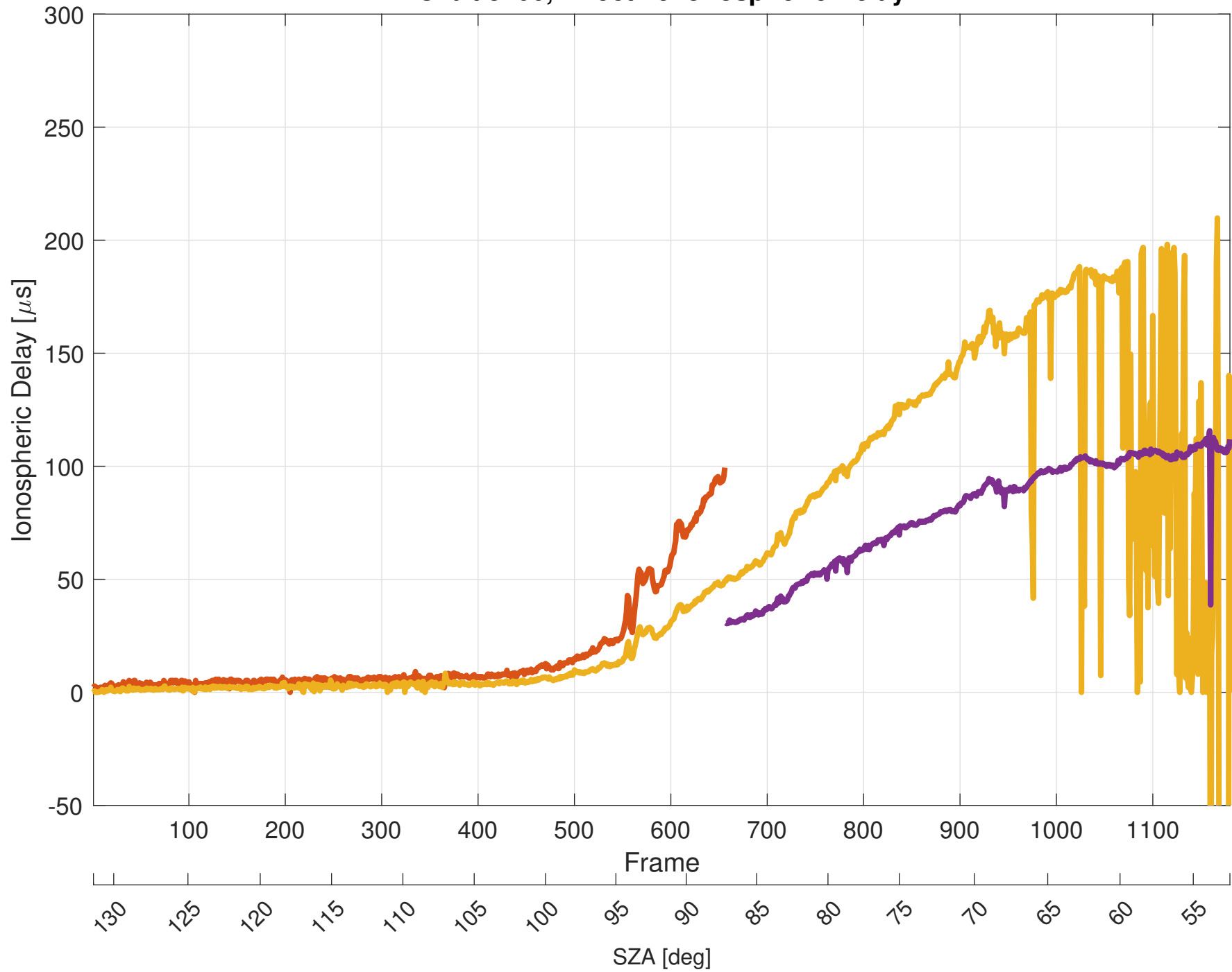
Orbit 3706, Effective Ionospheric Delay
