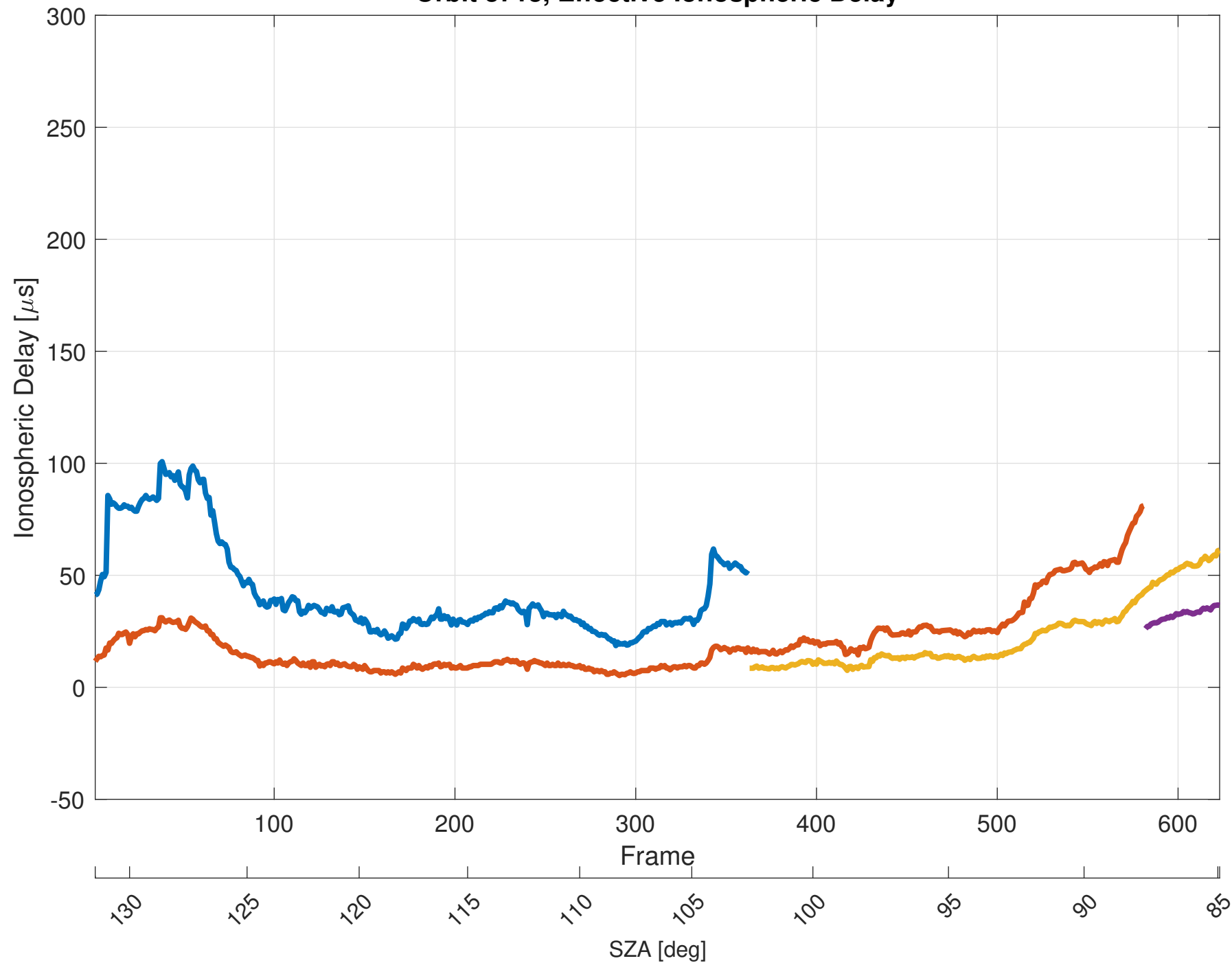
Orbit 3713, Effective Ionospheric Delay
