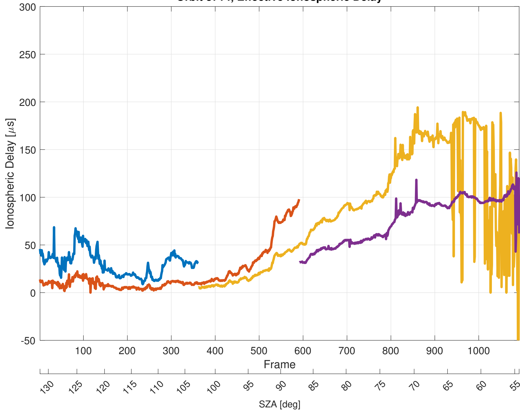
Orbit 3714, Effective Ionospheric Delay
