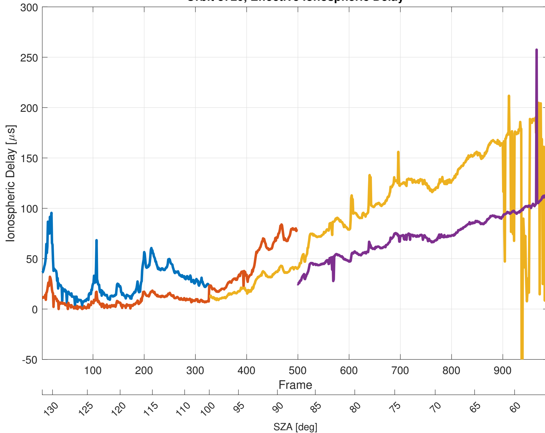
Orbit 3720, Effective Ionospheric Delay
