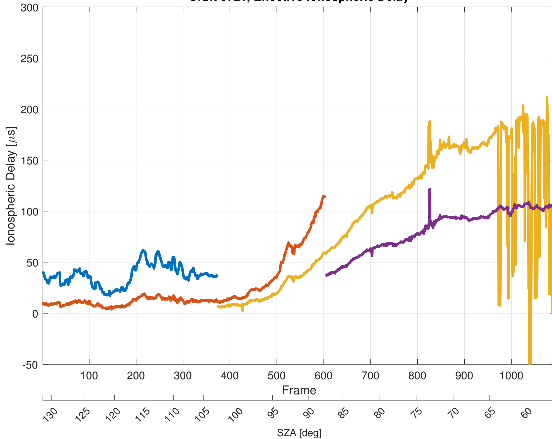
Orbit 3721, Effective Ionospheric Delay
