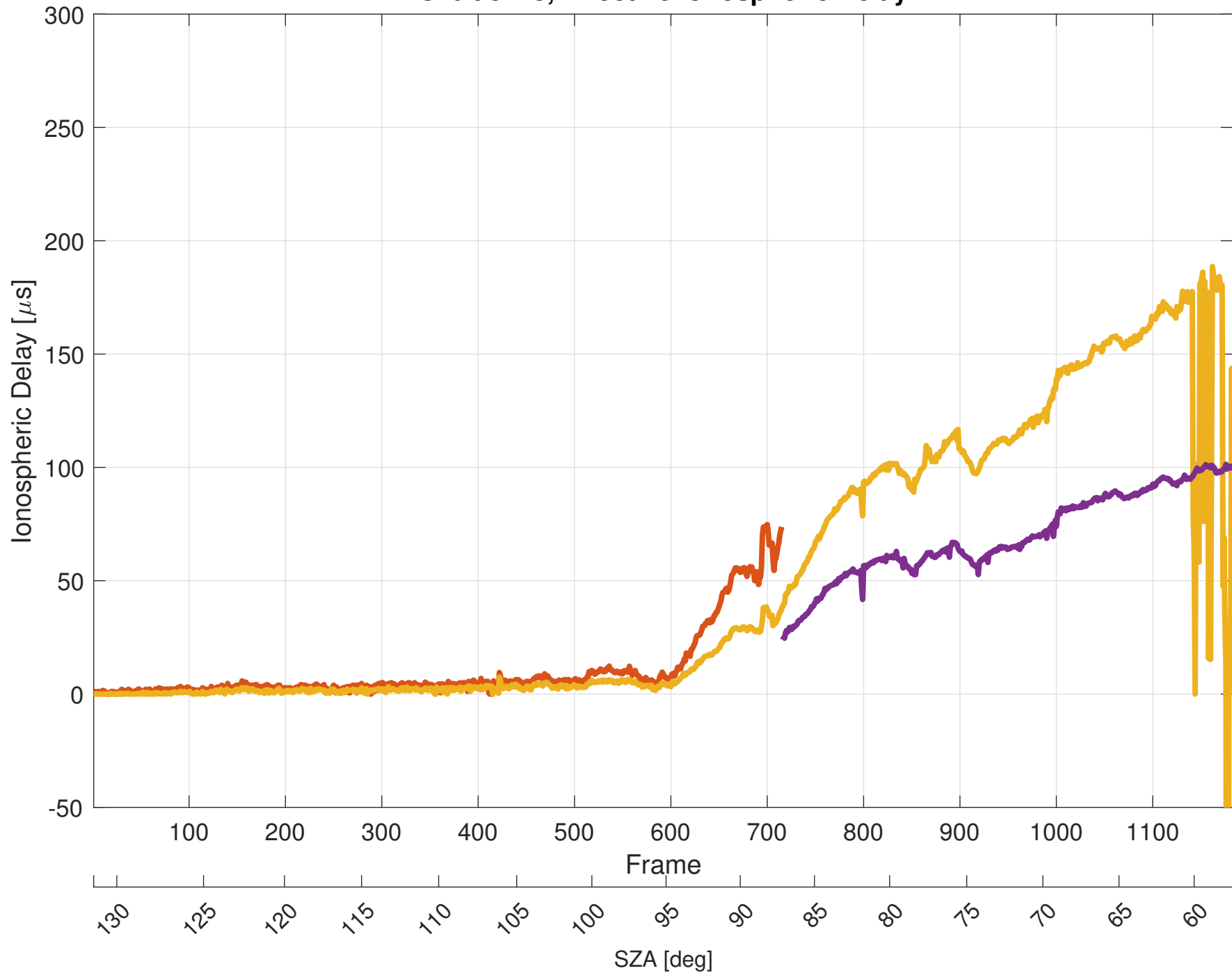
Orbit 3728, Effective Ionospheric Delay
