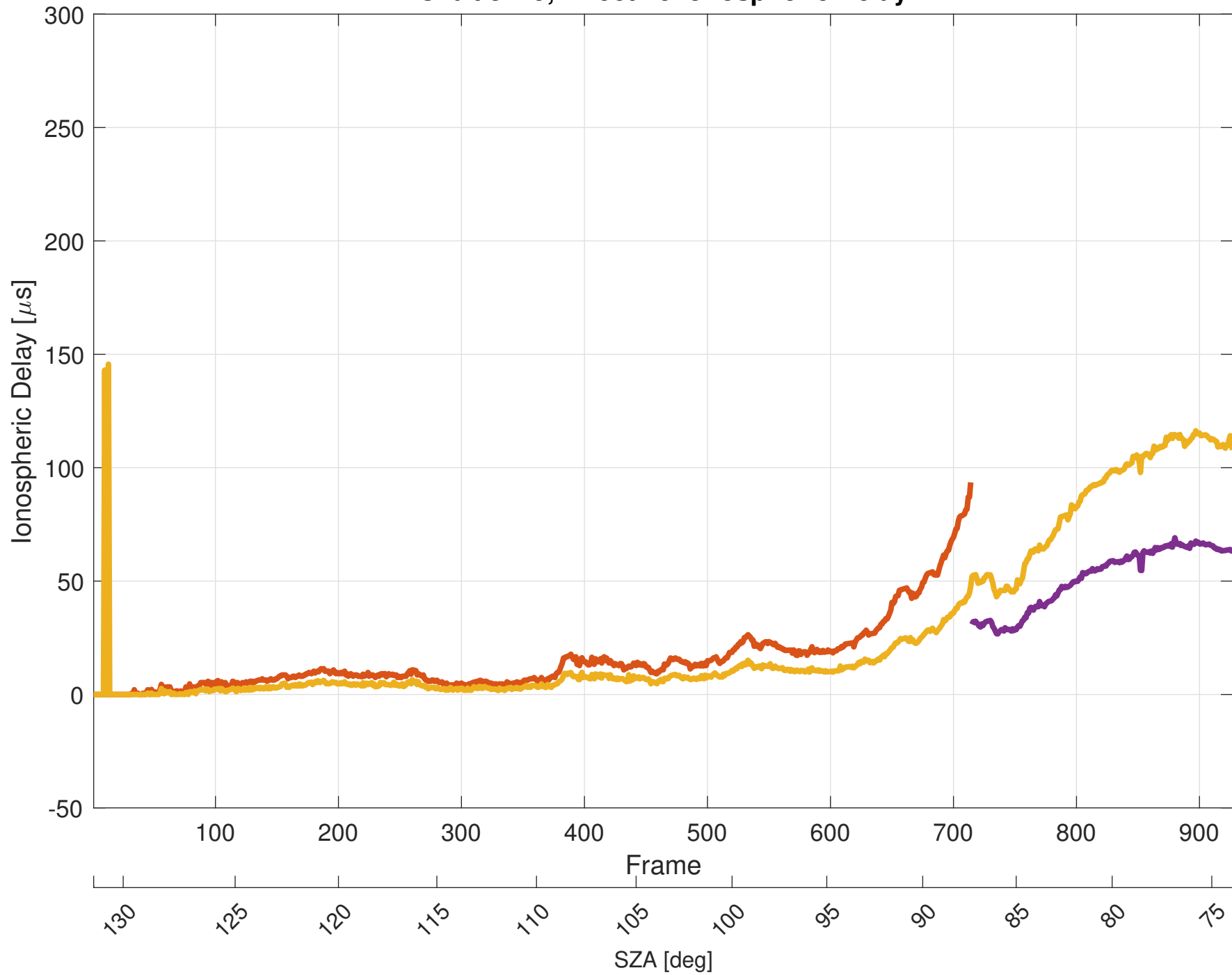
Orbit 3729, Effective Ionospheric Delay
