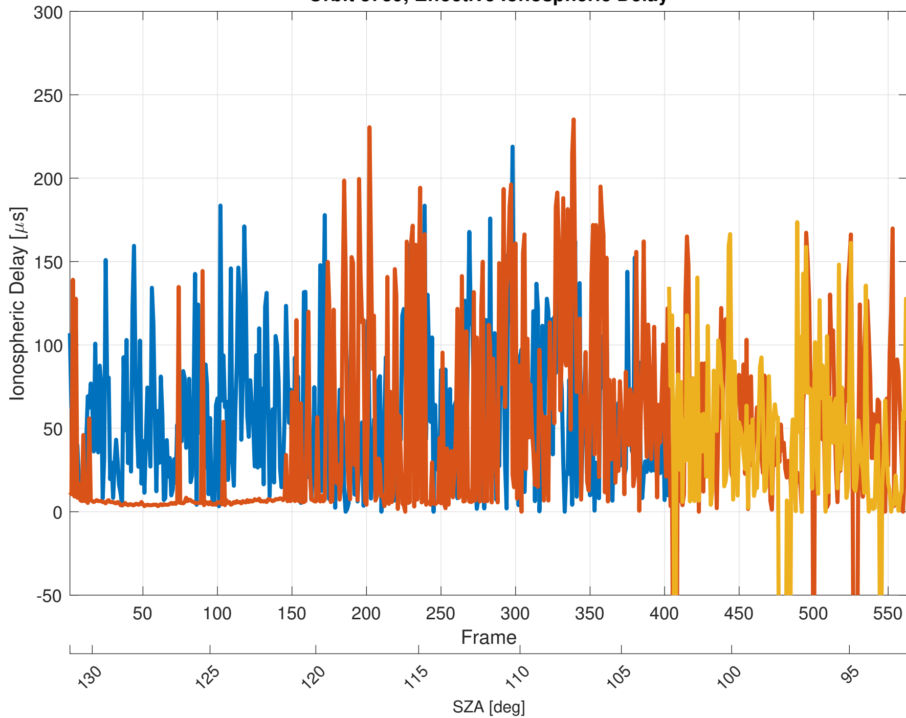
Orbit 3739, Effective Ionospheric Delay
