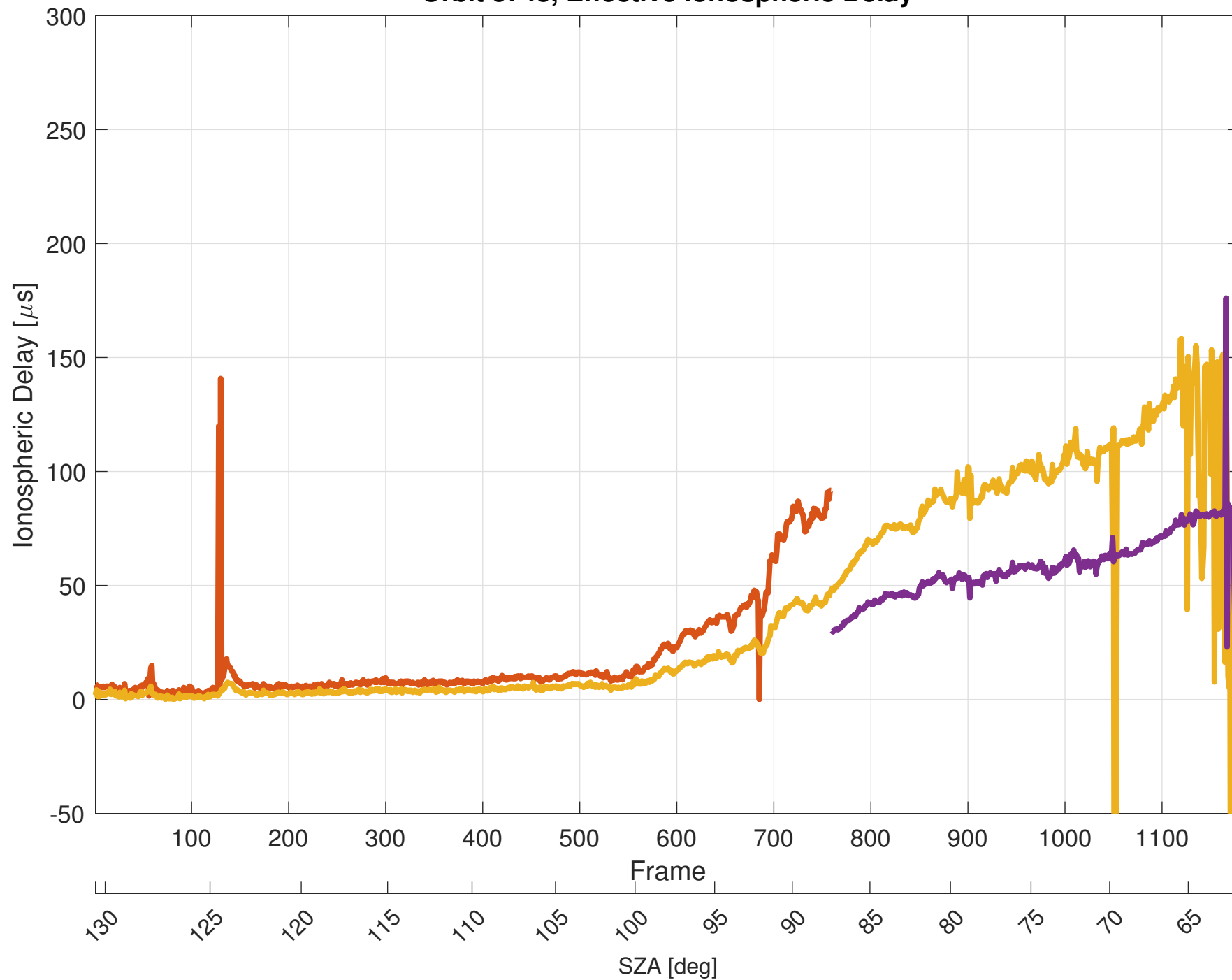
Orbit 3748, Effective Ionospheric Delay
