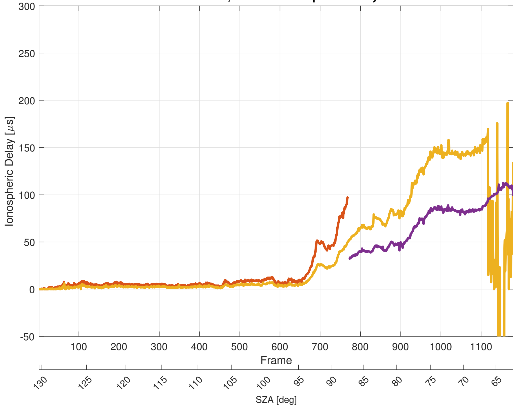
Orbit 3751, Effective Ionospheric Delay
