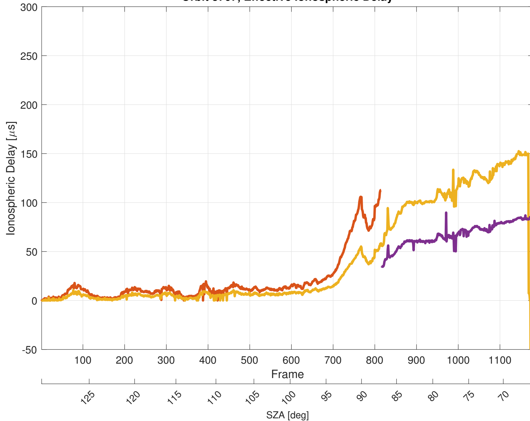
Orbit 3767, Effective Ionospheric Delay
