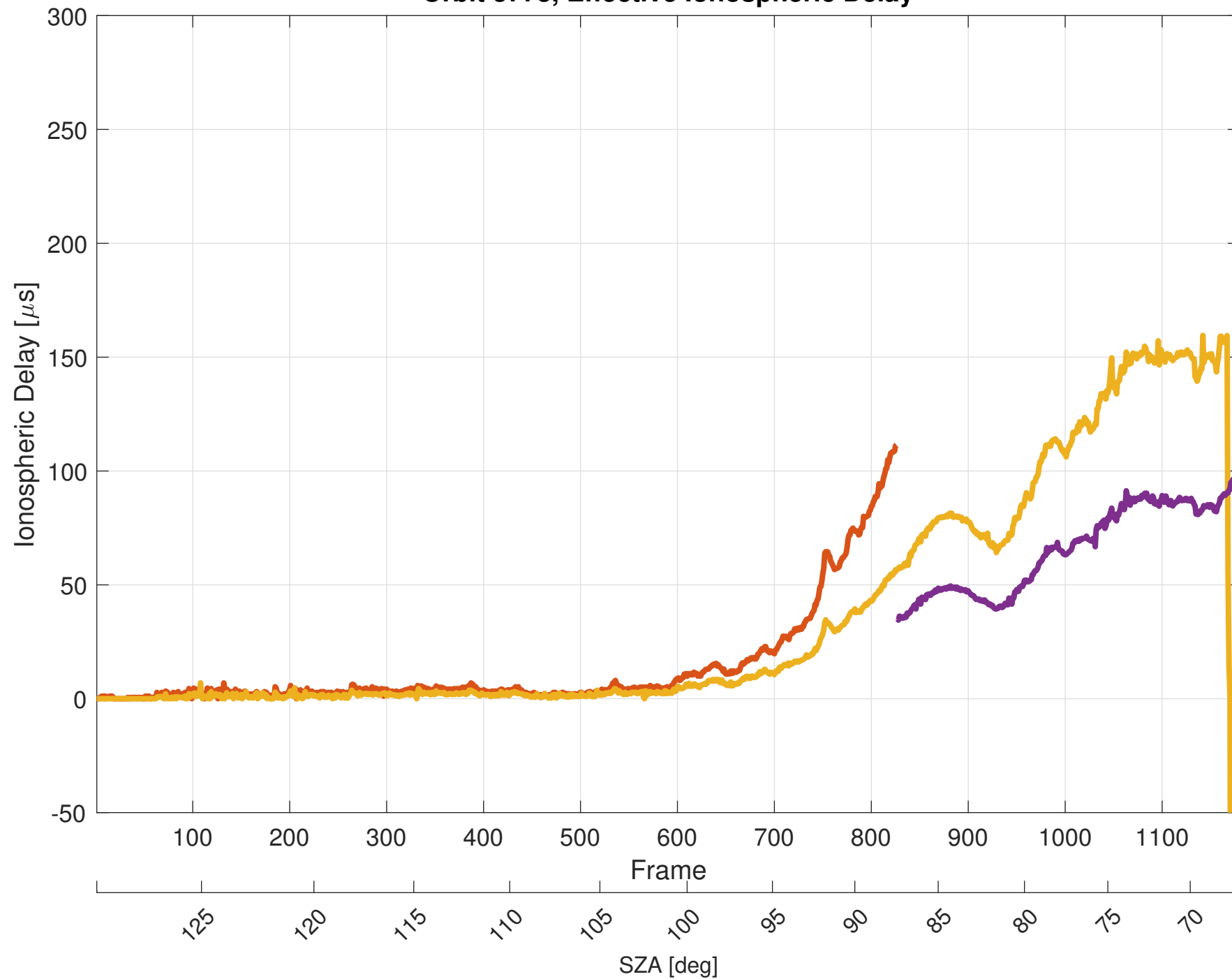
Orbit 3773, Effective Ionospheric Delay
