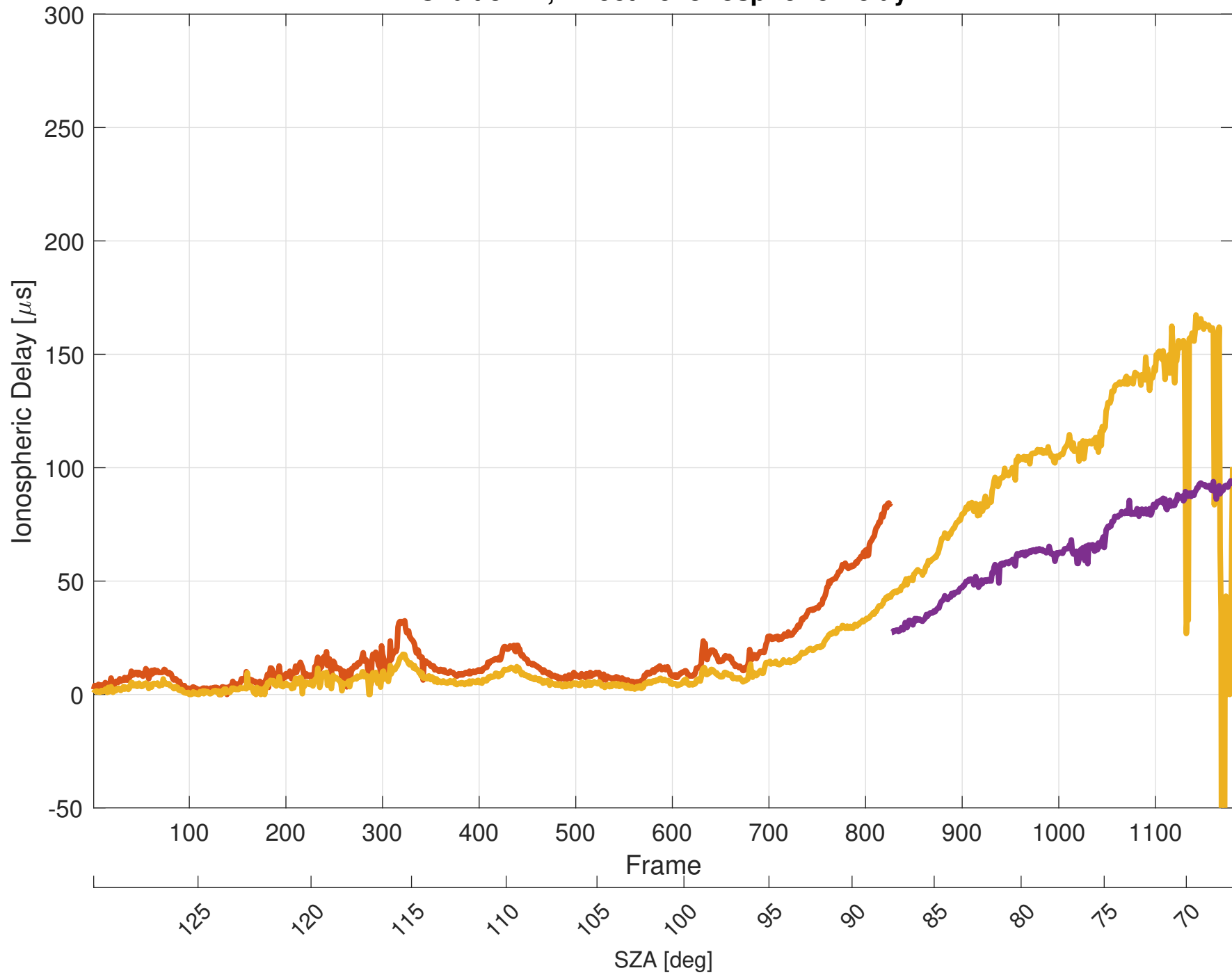
Orbit 3774, Effective Ionospheric Delay
