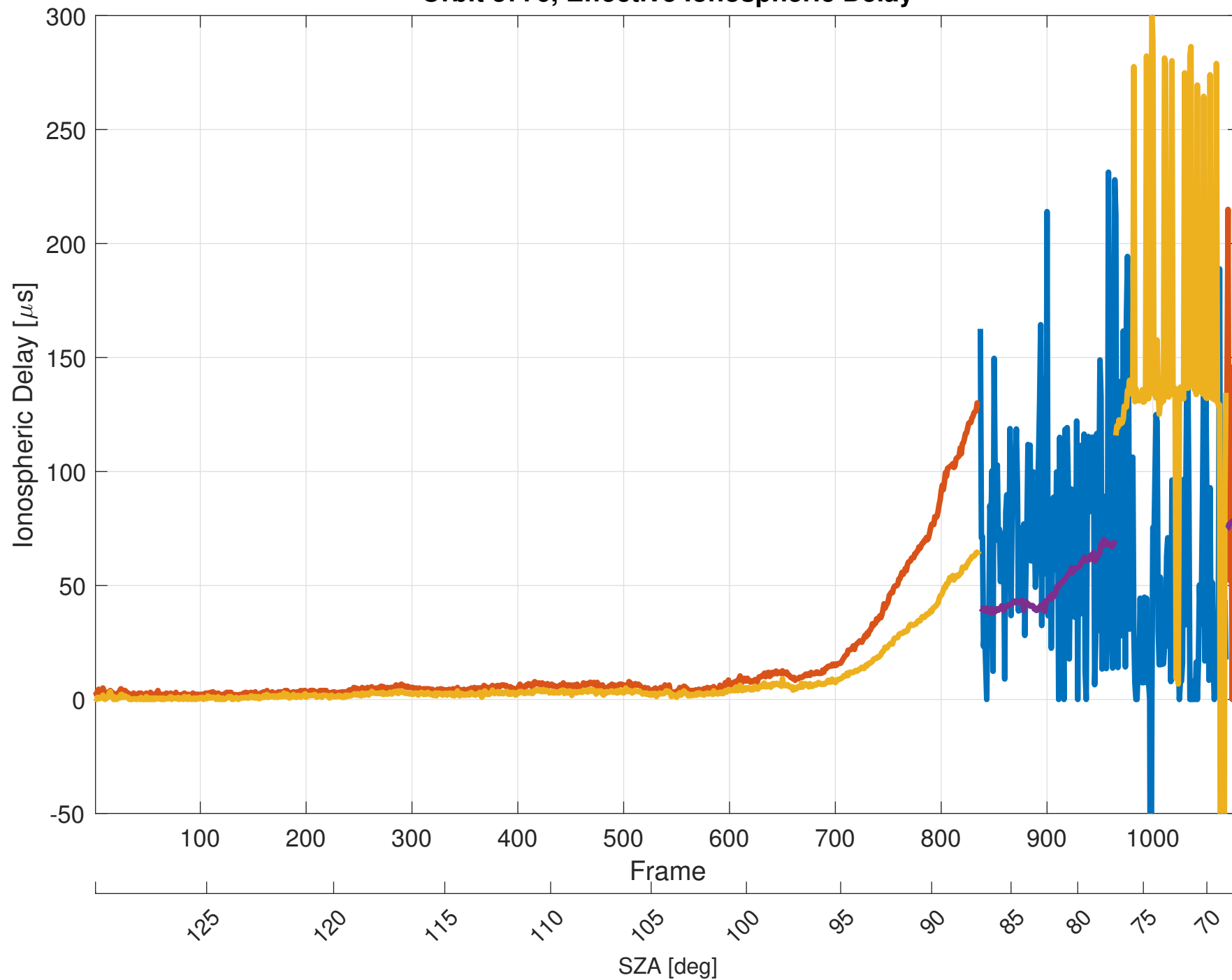
Orbit 3776, Effective Ionospheric Delay
