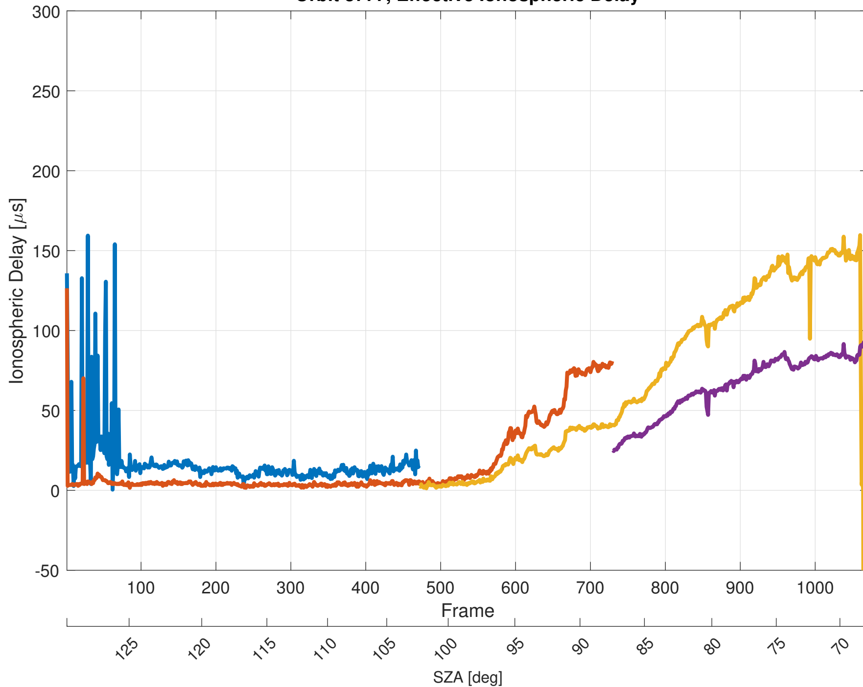
Orbit 3777, Effective Ionospheric Delay
