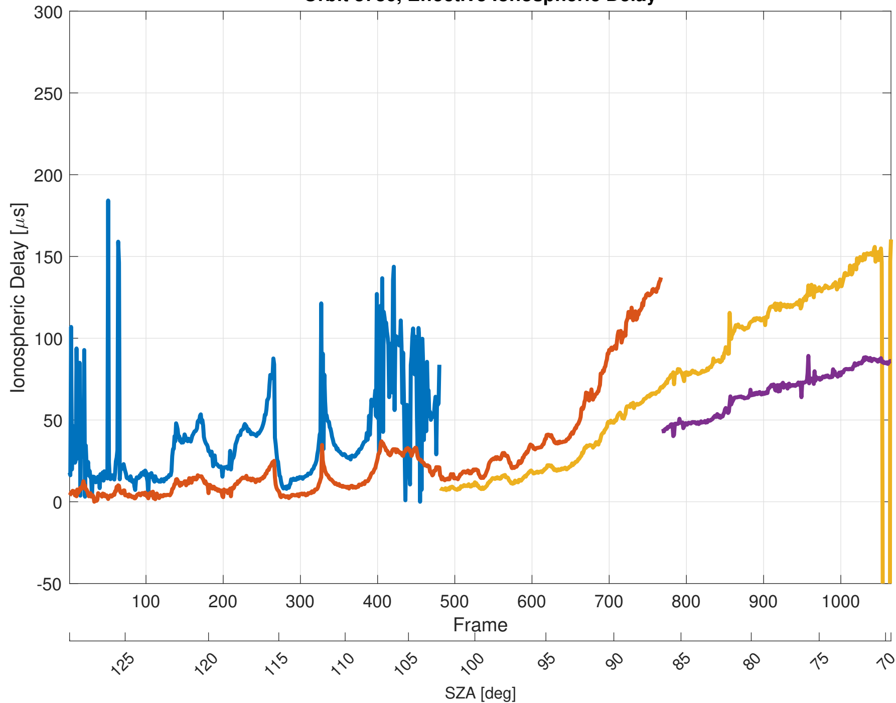
Orbit 3786, Effective Ionospheric Delay
