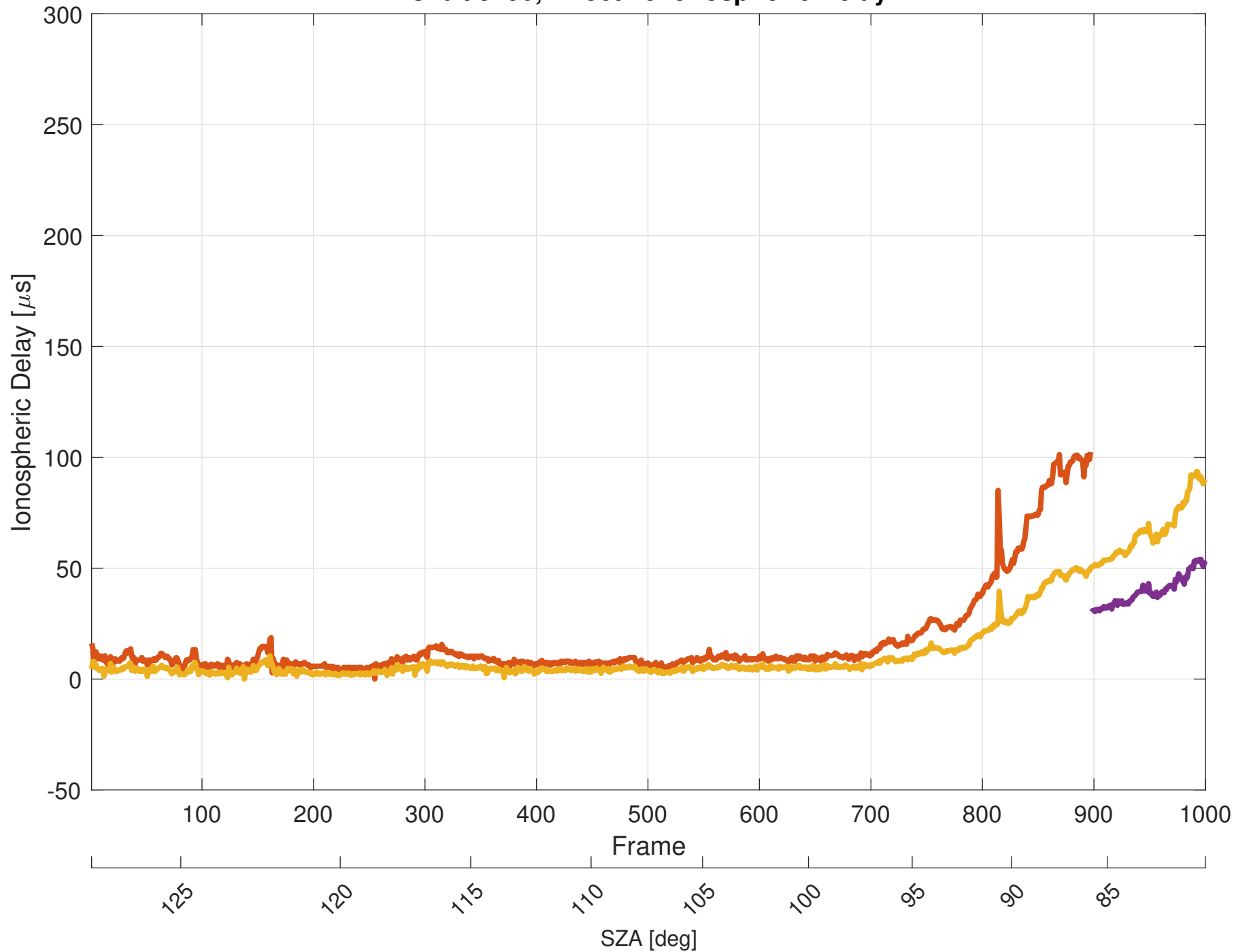
Orbit 3790, Effective Ionospheric Delay
