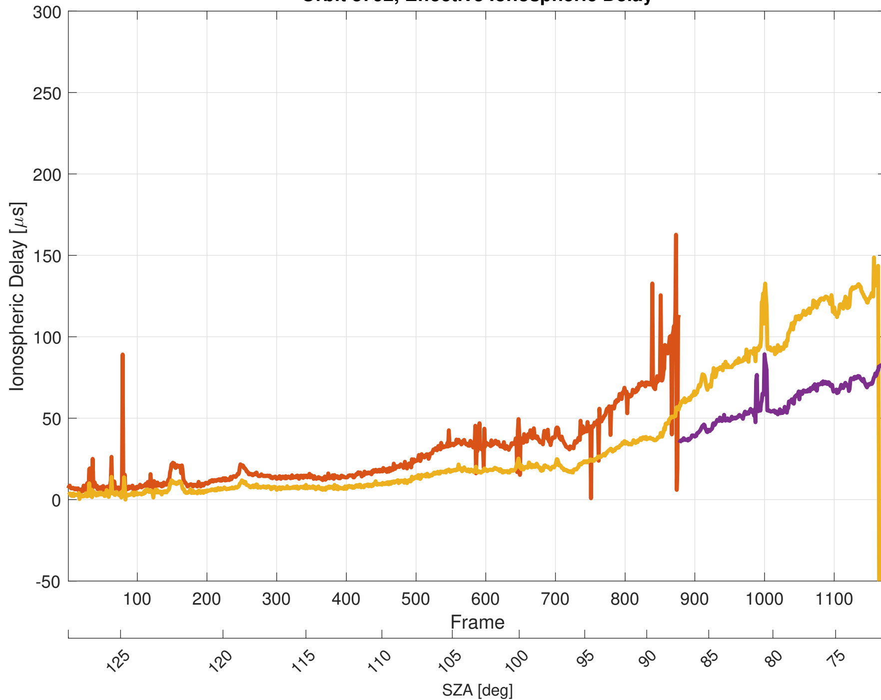
Orbit 3792, Effective Ionospheric Delay
