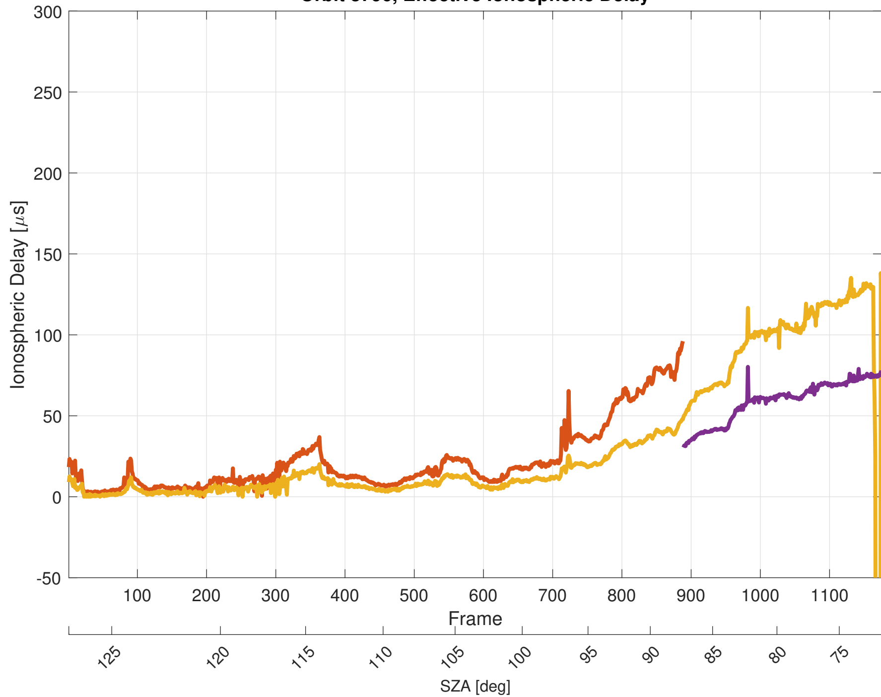
Orbit 3796, Effective Ionospheric Delay
