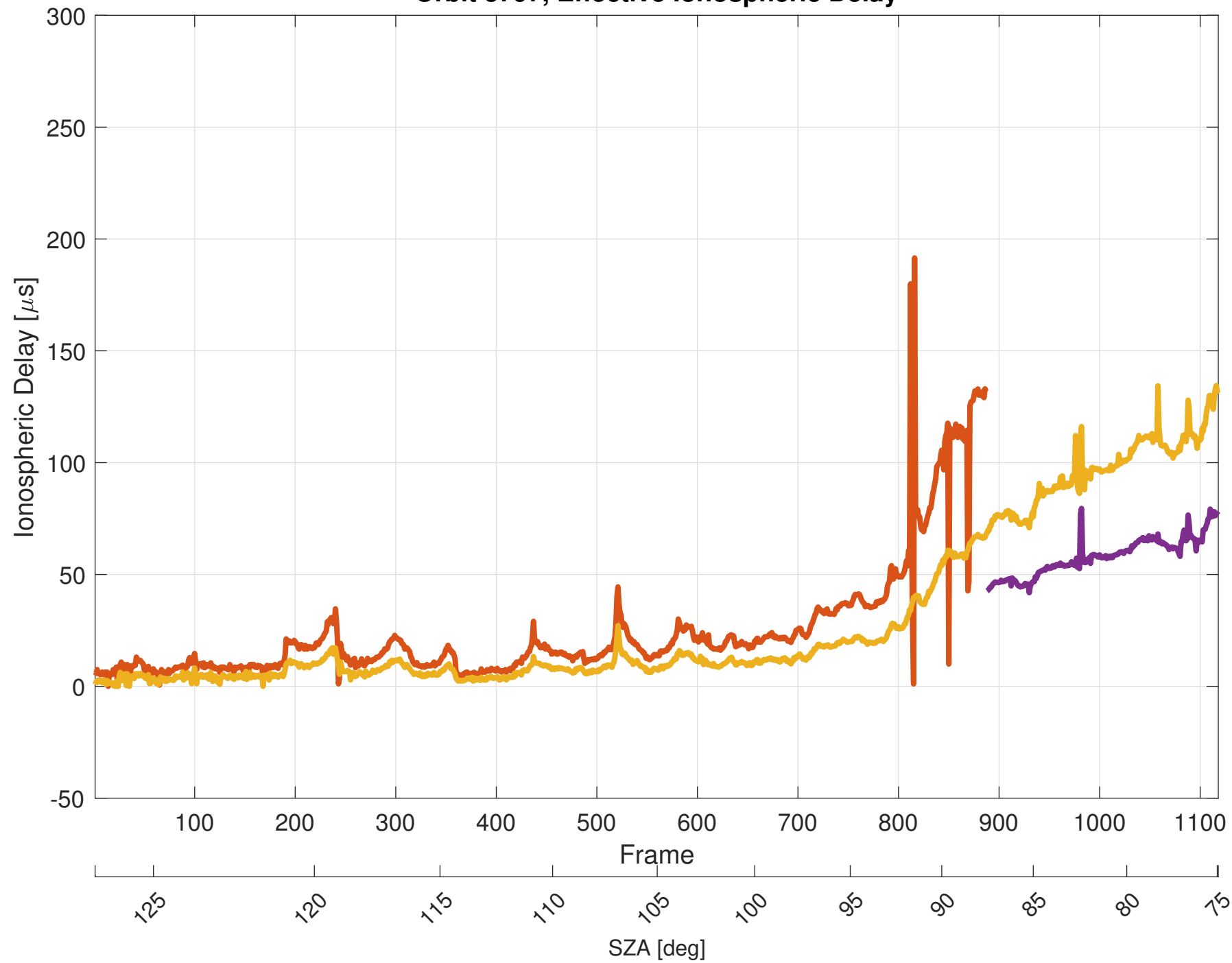
Orbit 3797, Effective Ionospheric Delay
