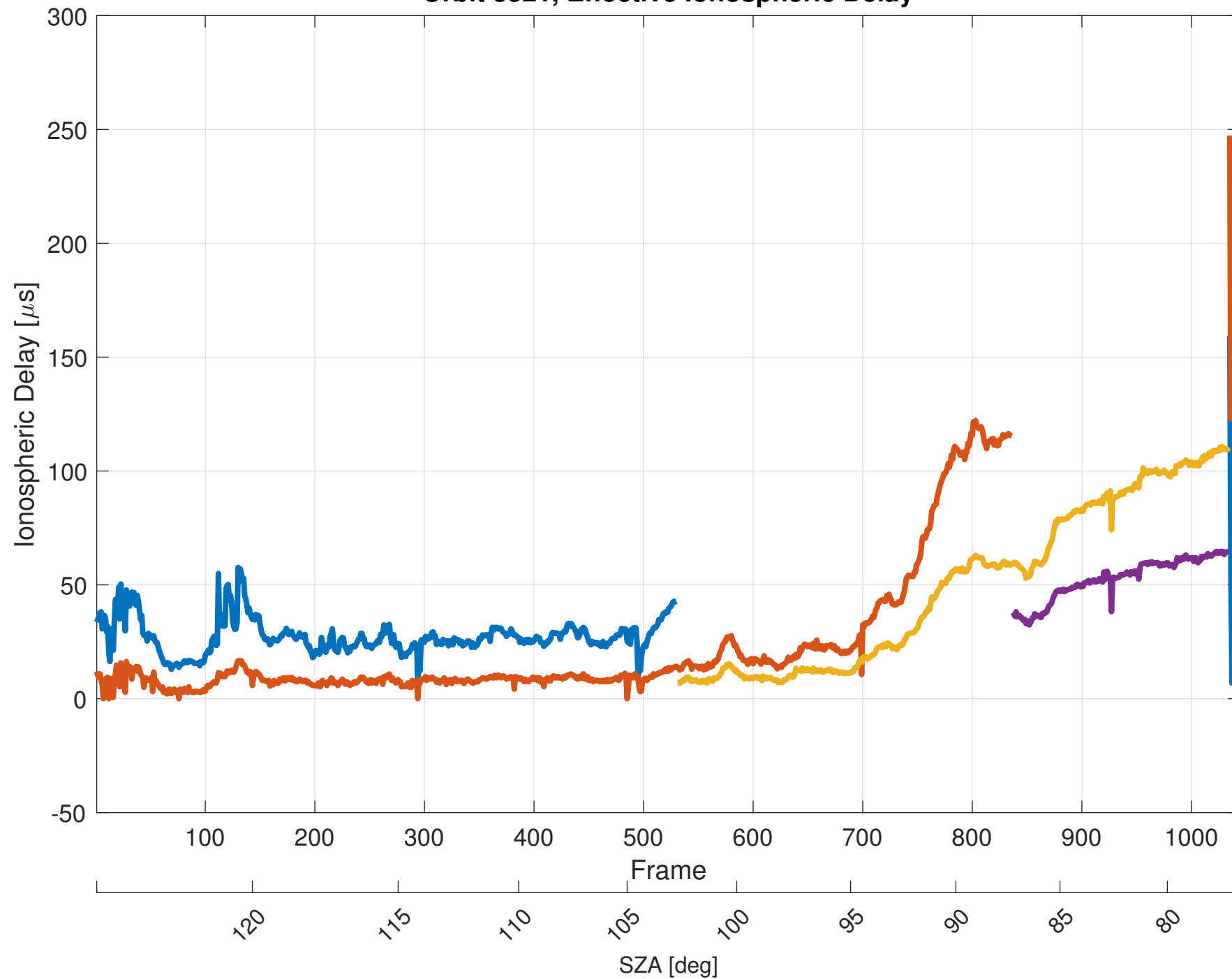
Orbit 3821, Effective Ionospheric Delay
