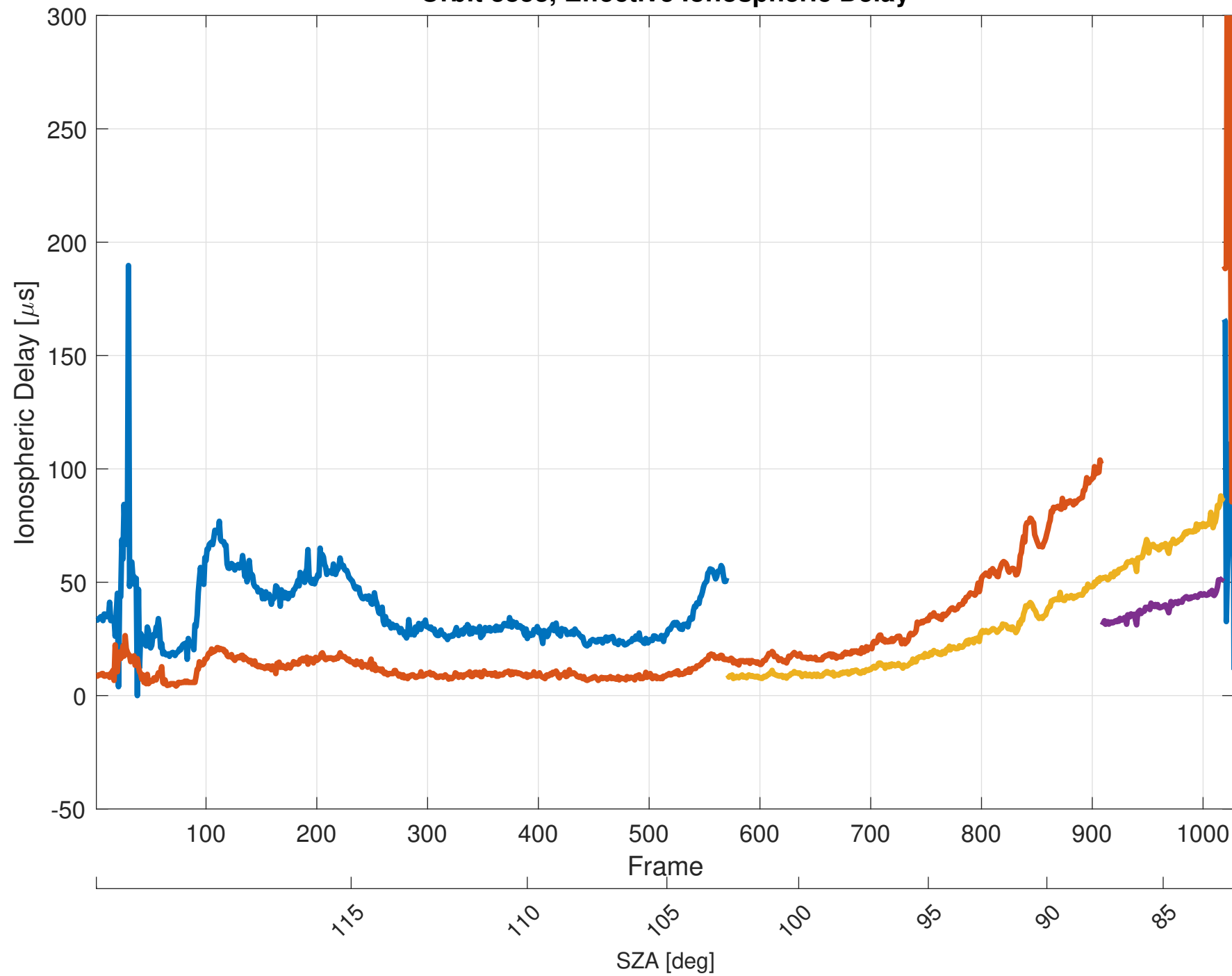
Orbit 3853, Effective Ionospheric Delay
