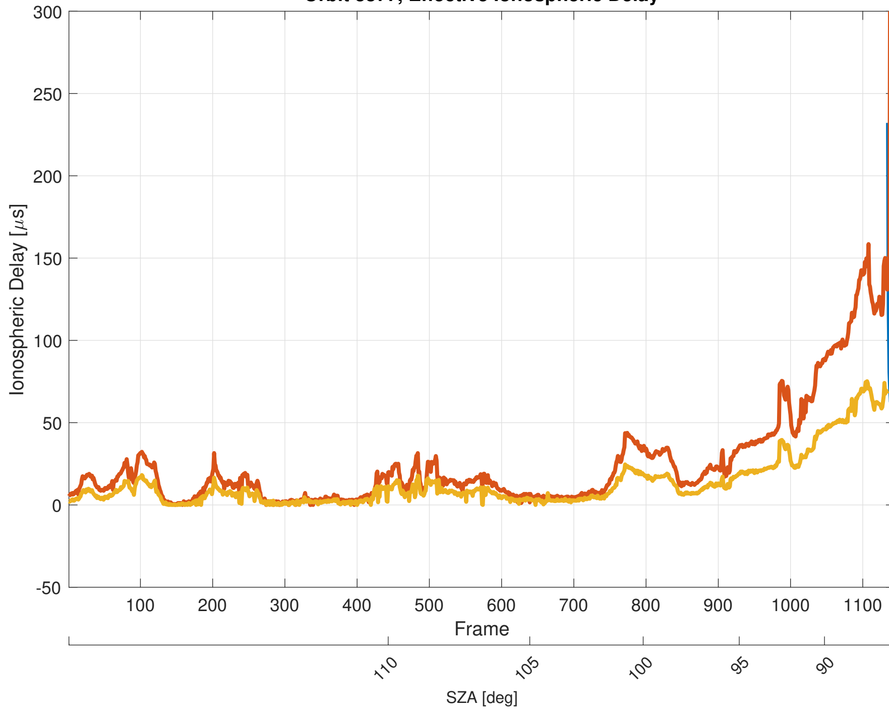
Orbit 3877, Effective Ionospheric Delay
