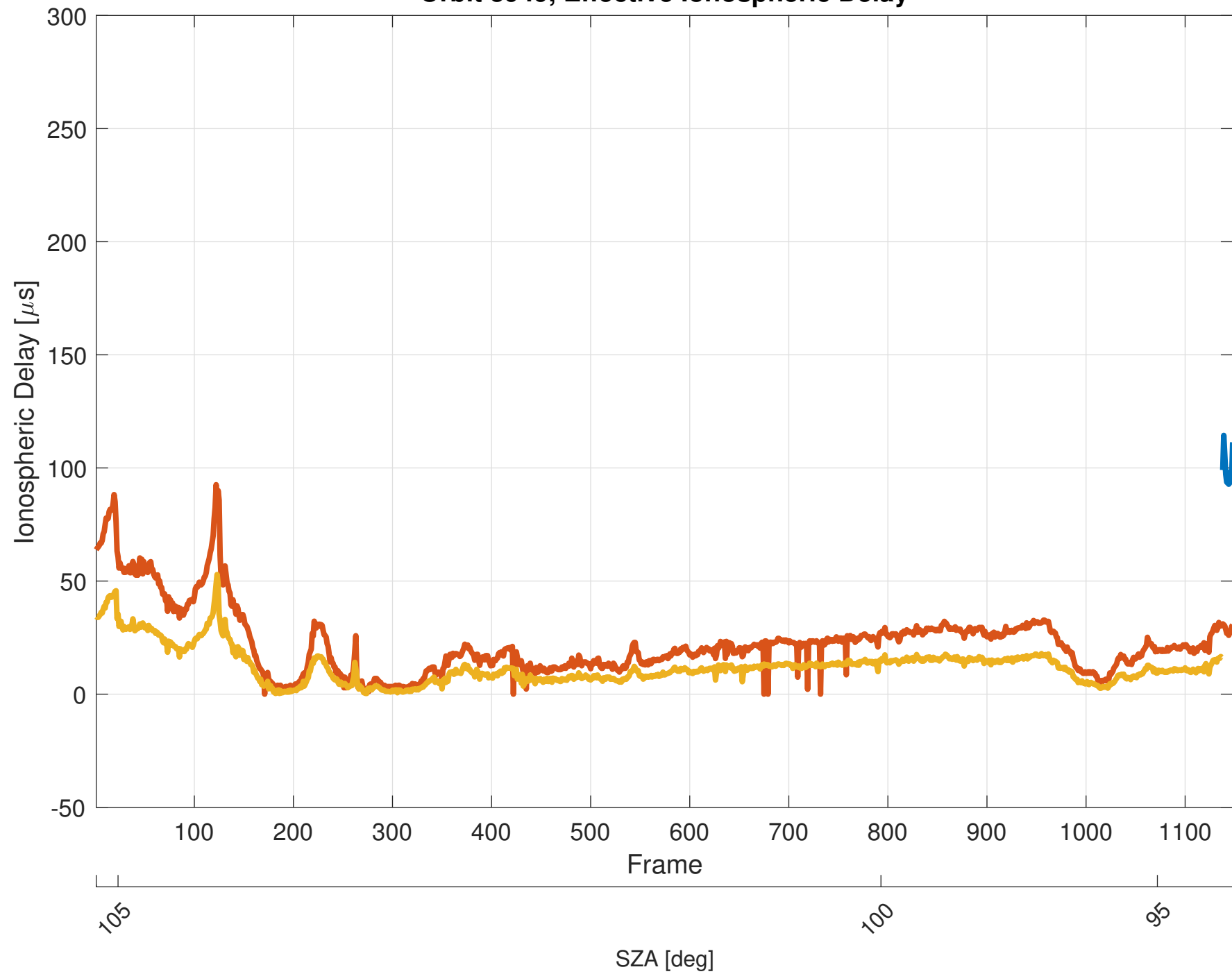
Orbit 3949, Effective Ionospheric Delay
