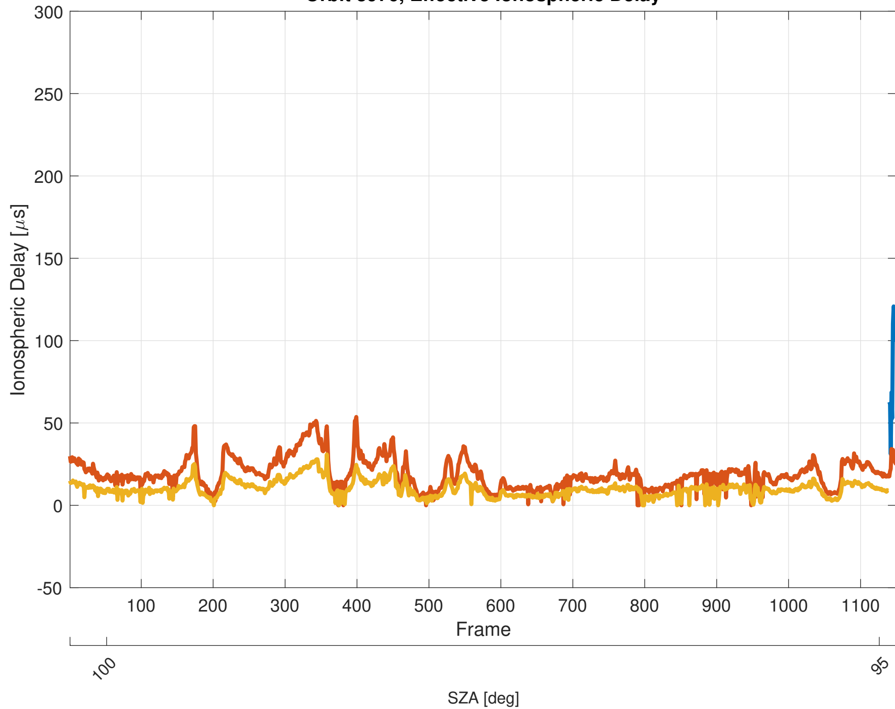
Orbit 3976, Effective Ionospheric Delay
