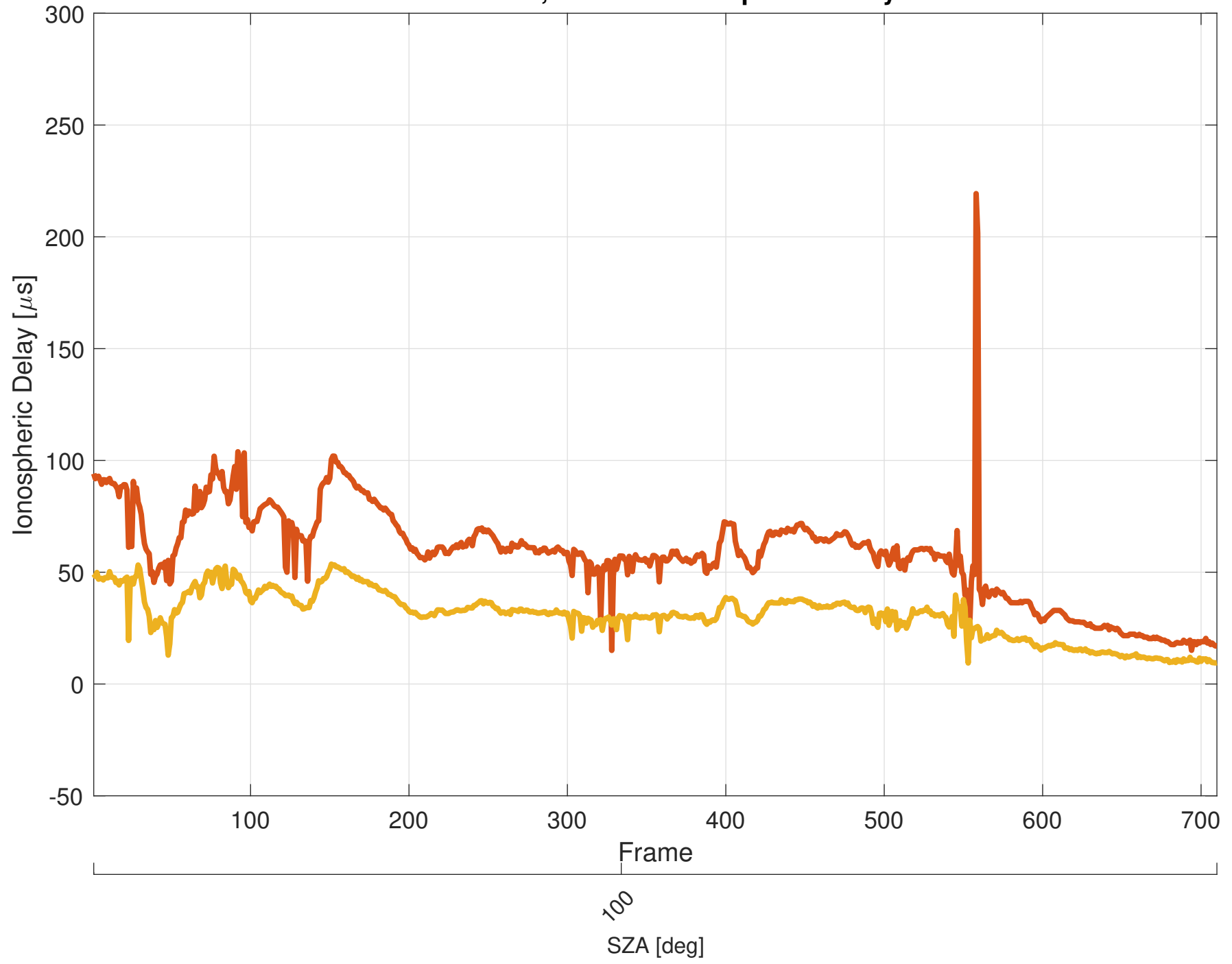
Orbit 3992, Effective Ionospheric Delay
